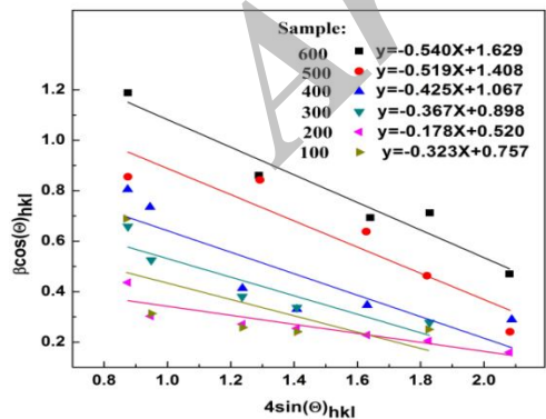
Fig. 4. Relation between βcosθ and 4sinθ (Williamson-Hall plots) with different TiO 2 content in composite.
