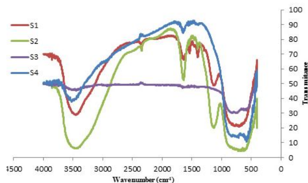
Fig. 9. FTIR spectra of the synthesized nano-alumina annealed at different reaction temperatures.
