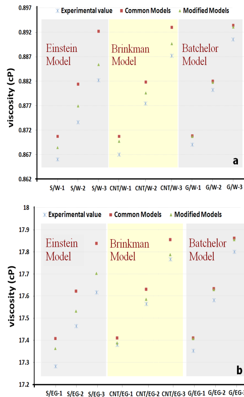
Fig. 3. Deviation of models and modified models with experimental viscosity of a) water base NF b) EG base NFs
