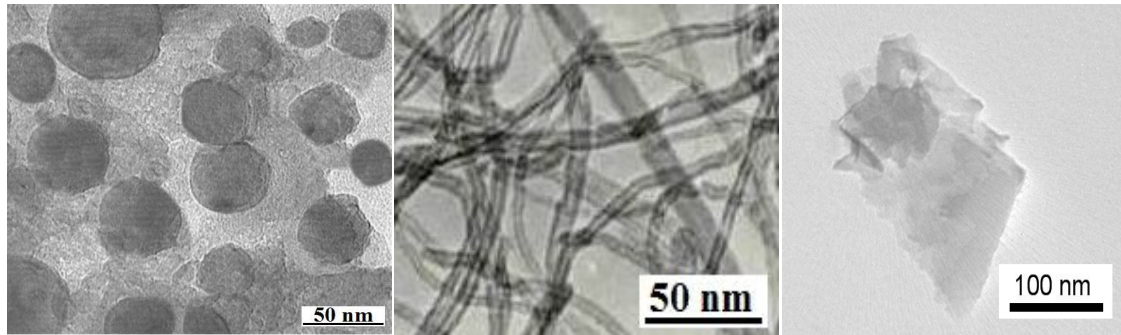
Fig. 1. TEM of a) SiO 2 b) CNT c) Graphene
