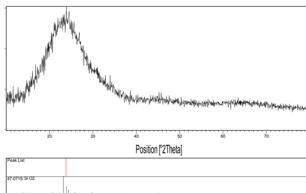
Fig. 3. XRD pattern of SiO 2 nanoparticles
