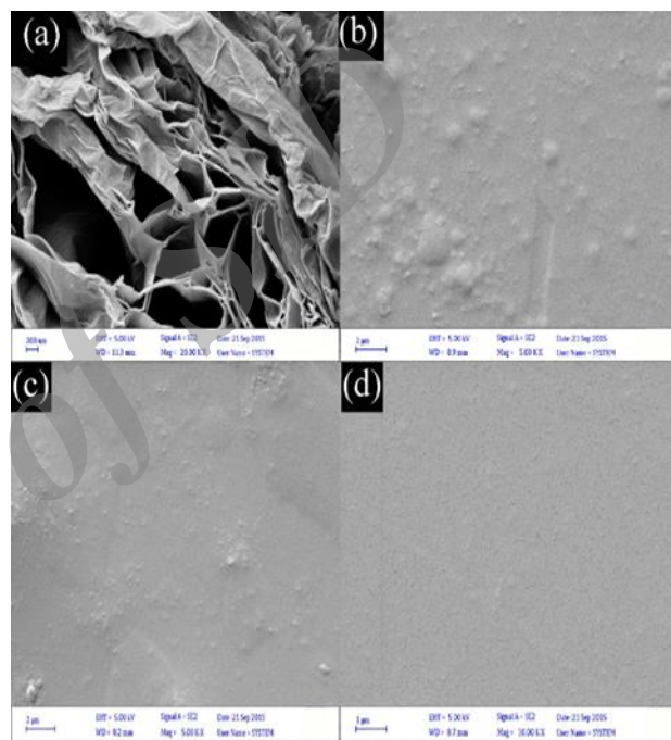
Fig. 3. SEM images of graphene nanosheets, S2, S5 and S6 samples.
