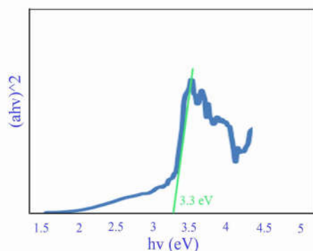
Fig. 9. Diffuse reflectance spectroscopy analysis of Fe 2 O 3 -TiO 2 nanoparticles
