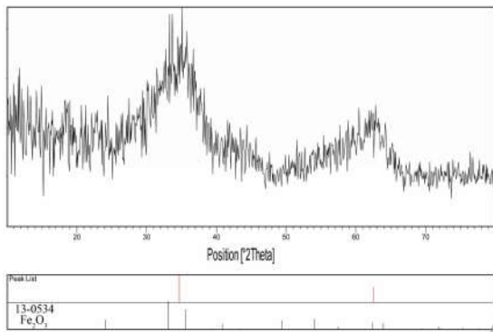
Fig. 2. XRD pattern of \text{Fe}_2\text{O}_3 nanoparticles
