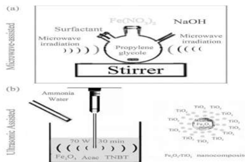
Fig. 1. Schematic of (a) microwave (b) ultrasonic
