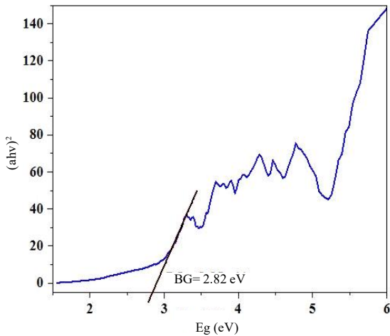
Fig. 7. The calculated band gap for 2-hydroxyacetophenone-CoFe 2 O 4
