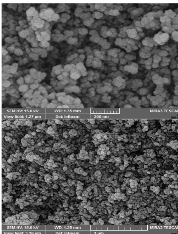
Fig. 3. SEM images of CoFe 2 O 4 stabilized by SDBS
