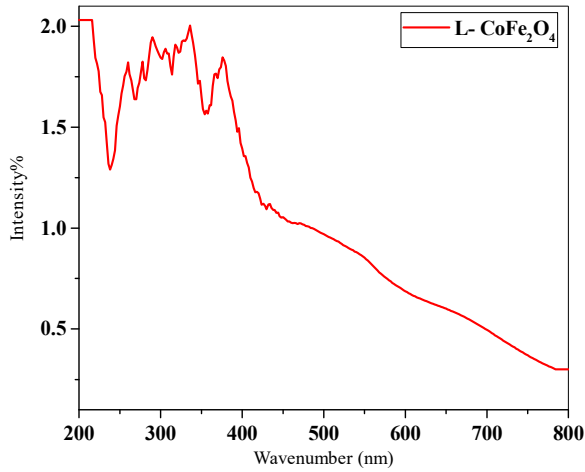
Fig. 6. UV-vis spectrum (DRS) for 2-hydroxyacetophenone-CoFe 2 O 4 nanoparticle.
