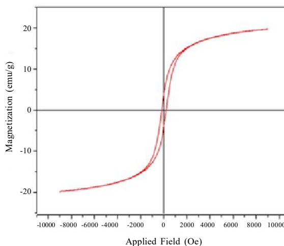
Fig. 5. Room temperature hysteresis loops of CoFe 2 O 4 nanoparticles
