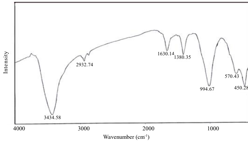
Fig. 2. IR spectrum for CoFe 2 O 4 synthesized by hydrothermal method
