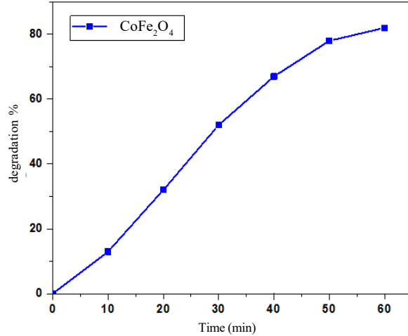
Fig. 8. Photodegradation of methylene blue by 2-hydroxyacetophenone-CoFe 2 O 4 nanoparticle, inset: Methylene blue after 60 minutes photodegradation in the presence of 2-hydroxyacetophenone-CoFe 2 O 4 nanoparticle
