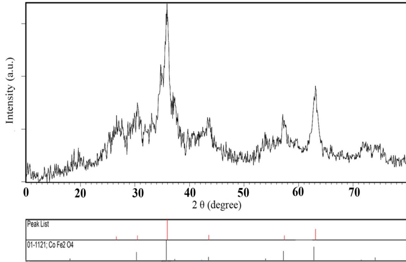
Fig. 1. XRD patterns for CoFe 2 O 4 synthesized by hydrothermal method.
