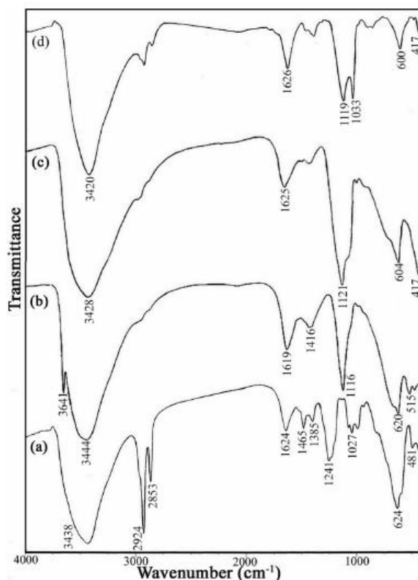
Fig. 3. FT-IR spectra of the typical samples before and after calcination: (a, c) SDS-0.01 and (b, d) CTAB-0.01.
