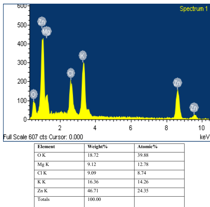
Fig. 3. EDX spectrum of ZnO NPs
