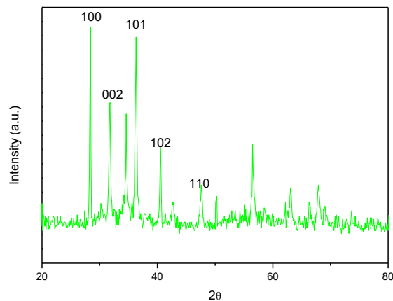
Fig. 1. XRD pattern of ZnO NPs
