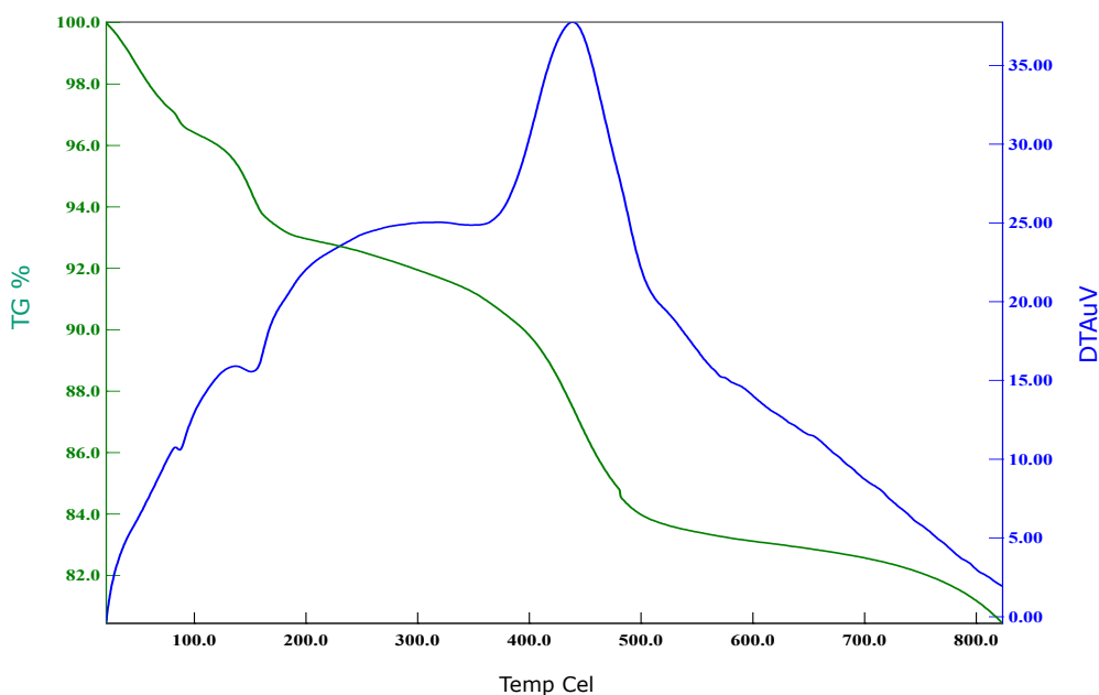
Fig .5 TG–DTA curves of the ZnO NPs
