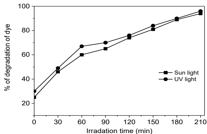
Fig. 6 Effect of different light source on photo catalytic degradation
