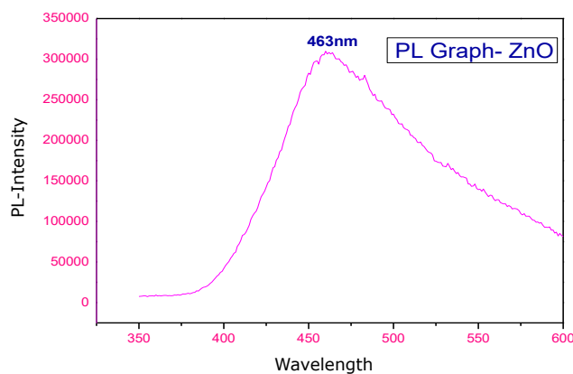
Fig. 4. Photoluminescence spectra of ZnO NPs
