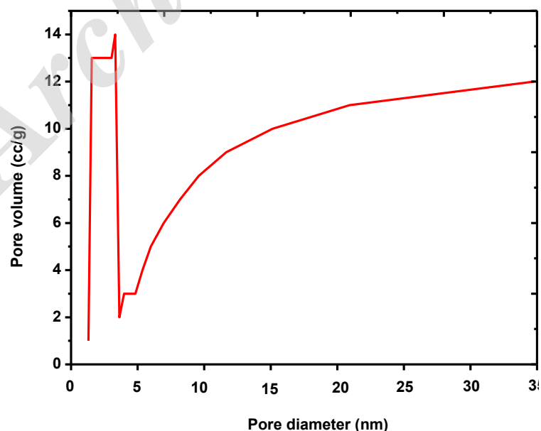
Fig. 7. BJH pore size distribution curves of synthesized CeVO 4 nanoparticles.
