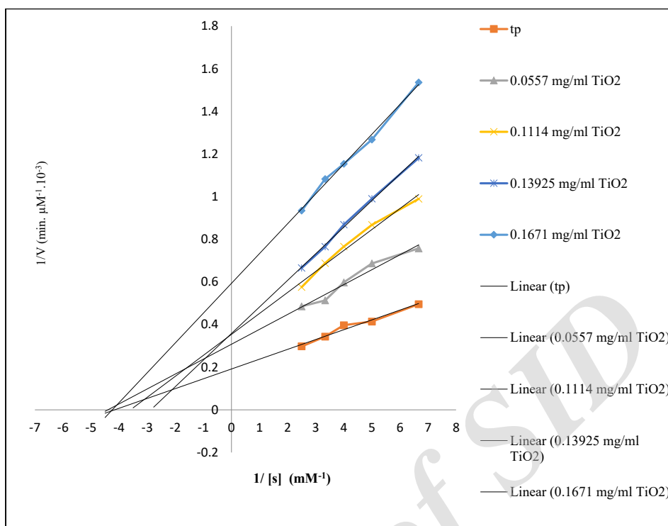
Fig. 3. Double reciprocal plots for trypsin in presence and absence of nano-TiO 2 at 30 °C, pH 8.0.
