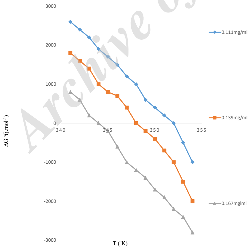
Fig. 9. Variation of Gibbs free energy vs. T (°K) at pH 3.0 .
