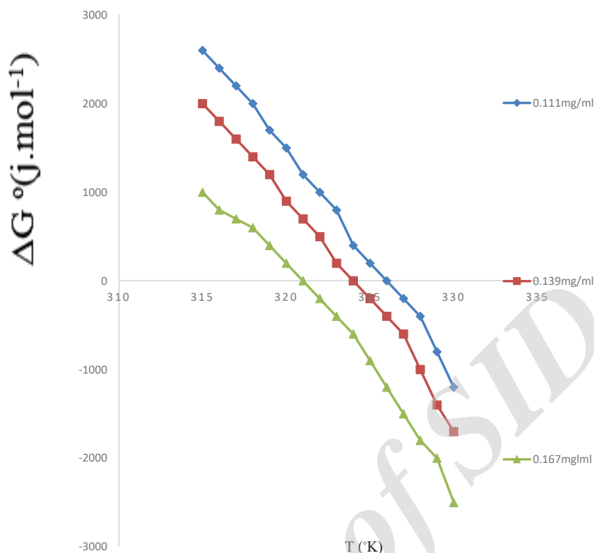
Fig. 10. Variation of Gibbs free energy vs. T (°K) at pH 7.25 .
