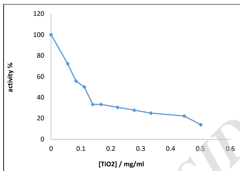
Fig. 2. The effect of TiO 2 NPs on the activity of trypsin.
