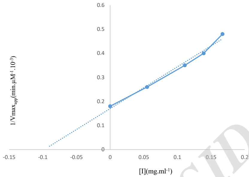
Fig. 5. (Secondary plot ) effect different concentration nano-TiO 2 on the activity trypsin at 30 °C, pH 8.0.
