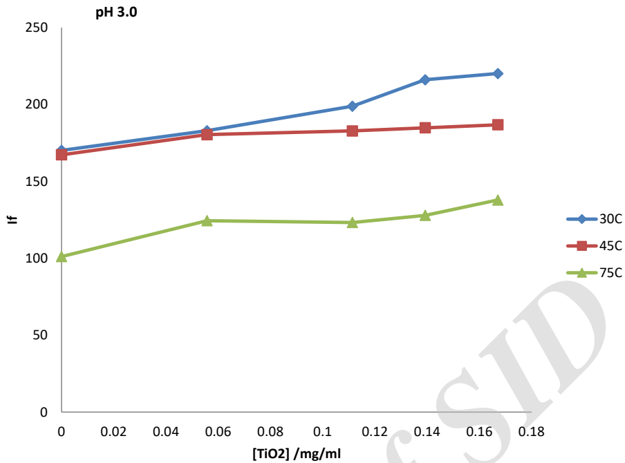
Fig. 7. The emission intensity of trypsin in presence and absence of nano-TiO 2 at pH 3.0 and temperatures of 30 °C, 45 °C, 75 °C
