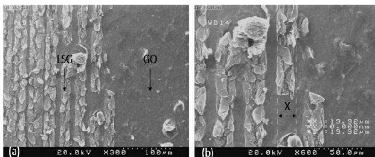
Fig. 2. SEM images of the laser scribed surface of graphene oxide at a low (a) and a high (b) magnification.
