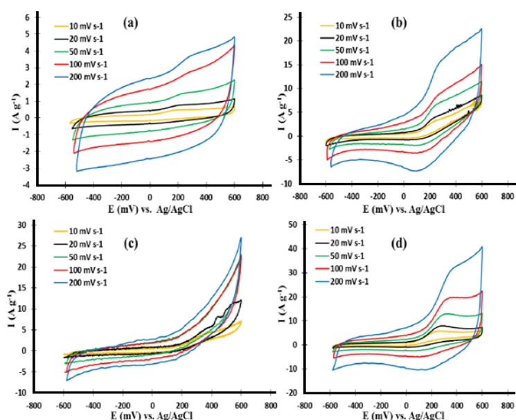
Fig. 6. The CV curves of pristine rGO (a) and MoS 2 /rGO composites with MoS 2 to rGO volume ratios of 1:100 (b), 1:75 (c) and 1:50 (d) at scan rate of 10, 20, 50, 100 and 200 mV s -1 in a voltage range of 600 and 600-mV in a three electrode system.
