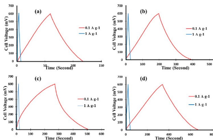
Fig. 7. Charge-discharge curves of pristine rGO (a) and MoS 2 /rGO composites with MoS 2 to rGO volume ratios of 1:100 (b), 1:75 (c) and 1:50 (d) at current densities of 0.1 and 1 A g -1 in a voltage range of 0–600mV in a three electrode system.
