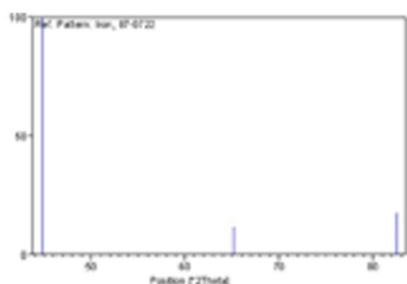
Fig. 6. XRD pattern of electrodeposited Fe nanowires
