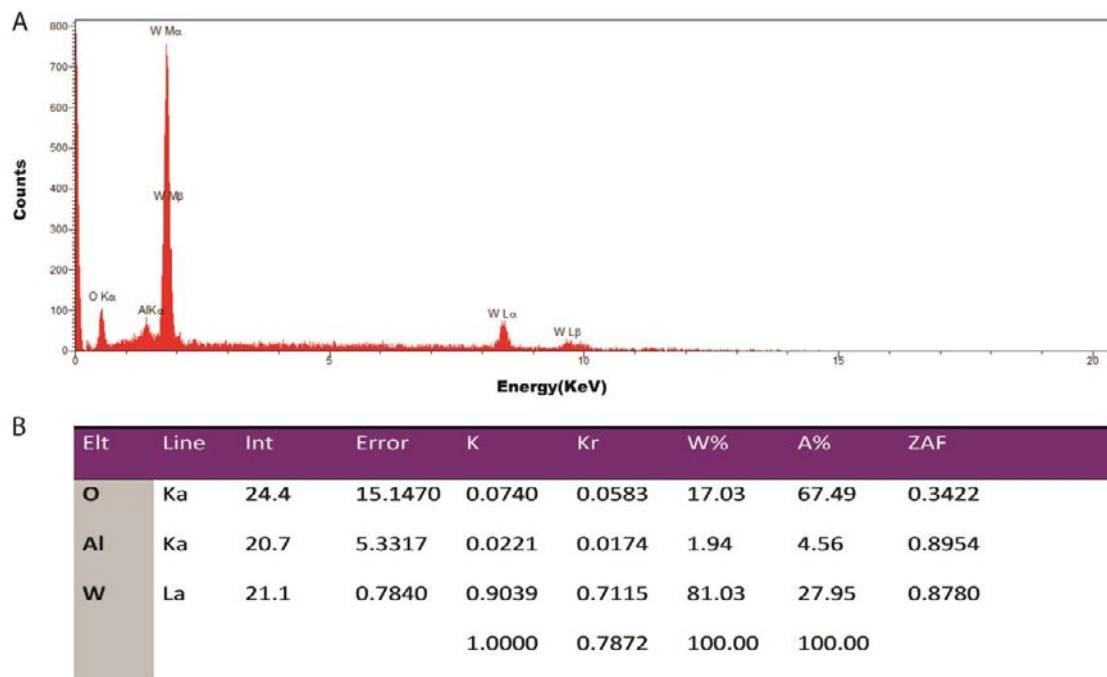
Fig. 3. EDS profile of WO 3 nanoparticles and quantitative analysis.
