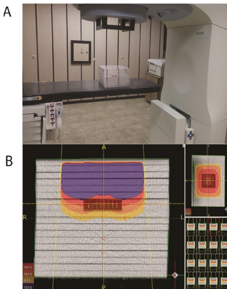
Fig. 1. Irradiation system (A) Multi-well micro plates containing the AGS cell are ready for in vitro tests. The AGS cells containing fresh medium alone or supplemented with 89.6 \mu g/mL of WO_3 NPs were seeded into low-attachment multi-well plates. Perspex phantom containing a micro titer plate was located on the treatment couch of the ONCOR Digital Medical Linear Accelerator, the same machine is used in daily clinical practice for the patients' radio therapeutic treatment and is subjected to specific quality assurance checks. (B) A CT scan was done in the set-up phase of the phantom containing the micro plate (in which wells were filled with culture medium) to optimize dose delivery, exactly the same as it's done for a patient. The irradiation system has ensured the delivery of a uniform dose to the yellow areas containing the micro plate, free of any doses. A Prowess Panther radiation therapy planning system was applied and customized with the geometric and dose-metric characteristics of an ONCOR Digital Medical Linear Accelerator.
