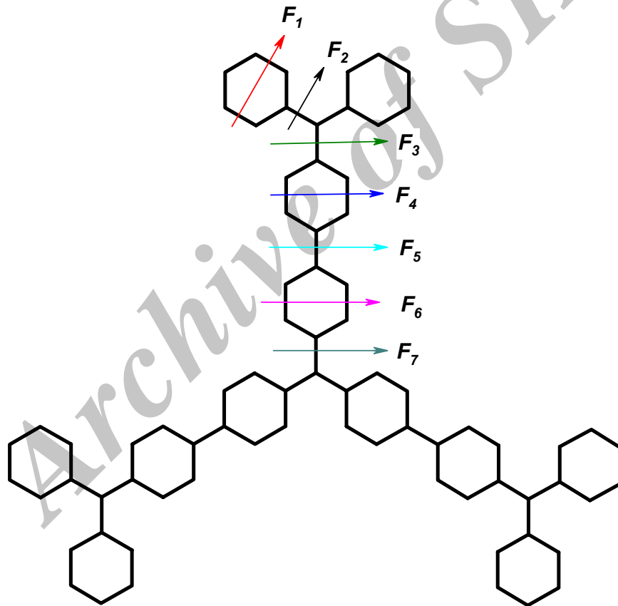
Figure 2. The nanostar dendrimer for n = 2 .
