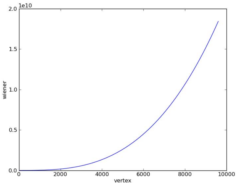
Figure 7. The Wiener Index Versus Vertex.
