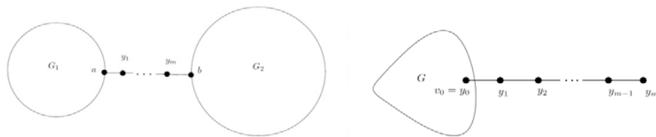
Figure 1. Graphs G(m) and G_1(m)G_2 , respectively.
