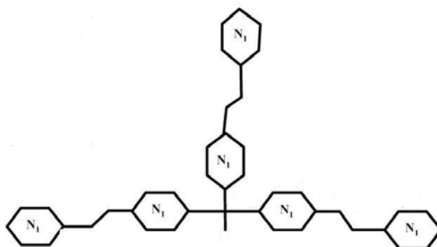
Figure 2. The kernel of NS_1[3] .
