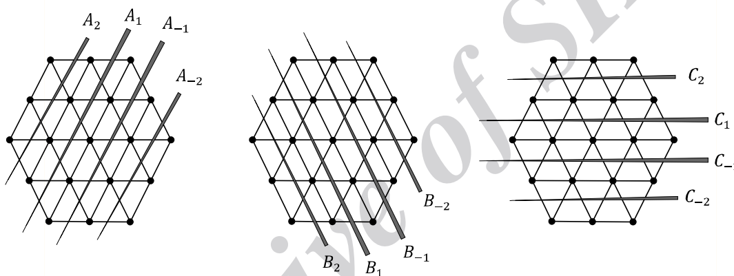
Figure 6: Edge Cuts of HX(3) .
