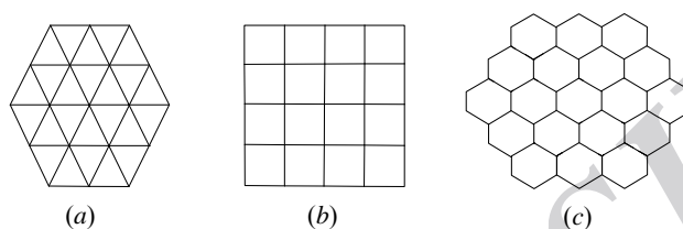
Figure 4: Three Regular Tessellations Composed of the Same Kind of Regular Polygons: (a) Equilateral Triangles (b) Squares and (c) Hexagons.
