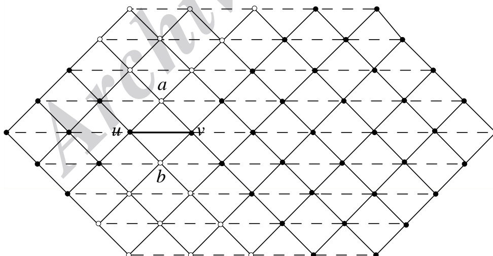
Figure 9: The Vertices Equidistant to u and v are Represented by Hollow Vertices.
