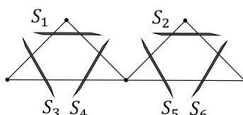
Figure 2: S_1, S_2, S_3, S_4, S_5, S_6 are Edge Cuts of \Delta S_5 .
