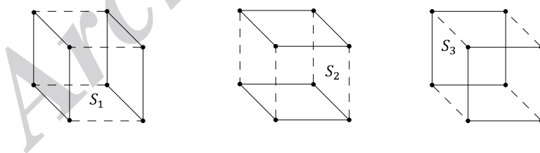
Figure 1: S_1, S_2, S_3 are Edge Cuts of Q_3 .
