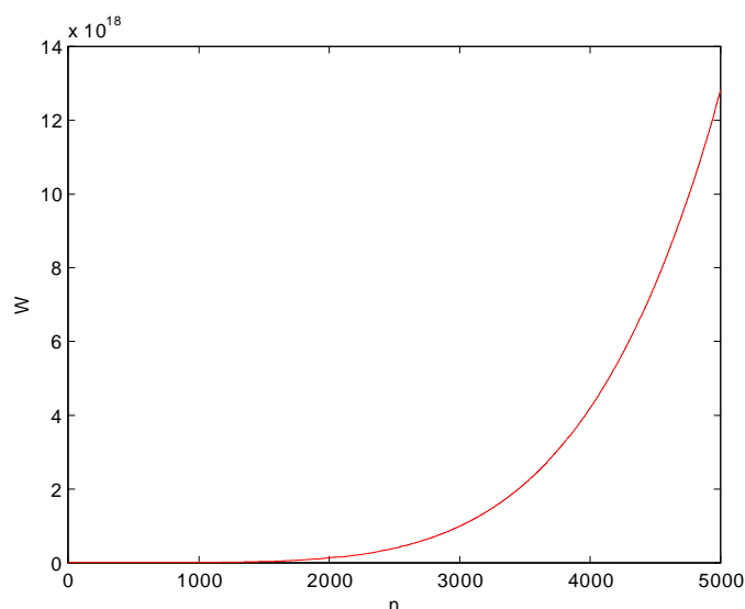
Figure 7: Graph Representation of W(HX(n)) .
