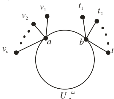
Figure 2. Graph U_n^{r,s} .
