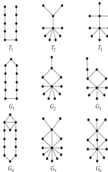
Figure 6. Graphs with the same indices.
