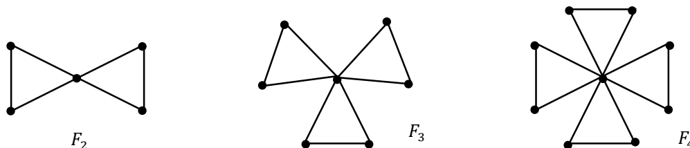
Figure 3. Graphs F_2 , F_3 and F_4 .
