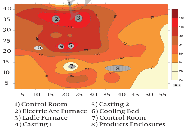
Figure 2. Isosonic Map of Metal Melting Factory
