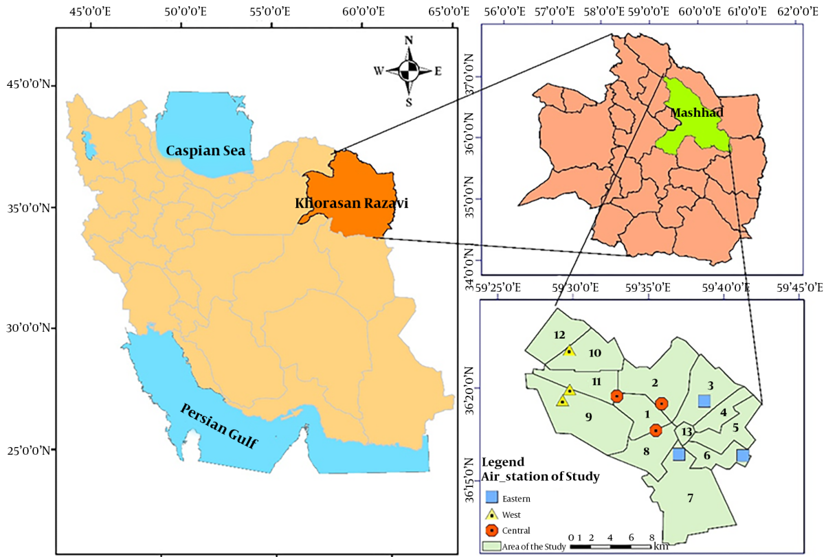
Figure 1. Study area and air quality measurement stations
