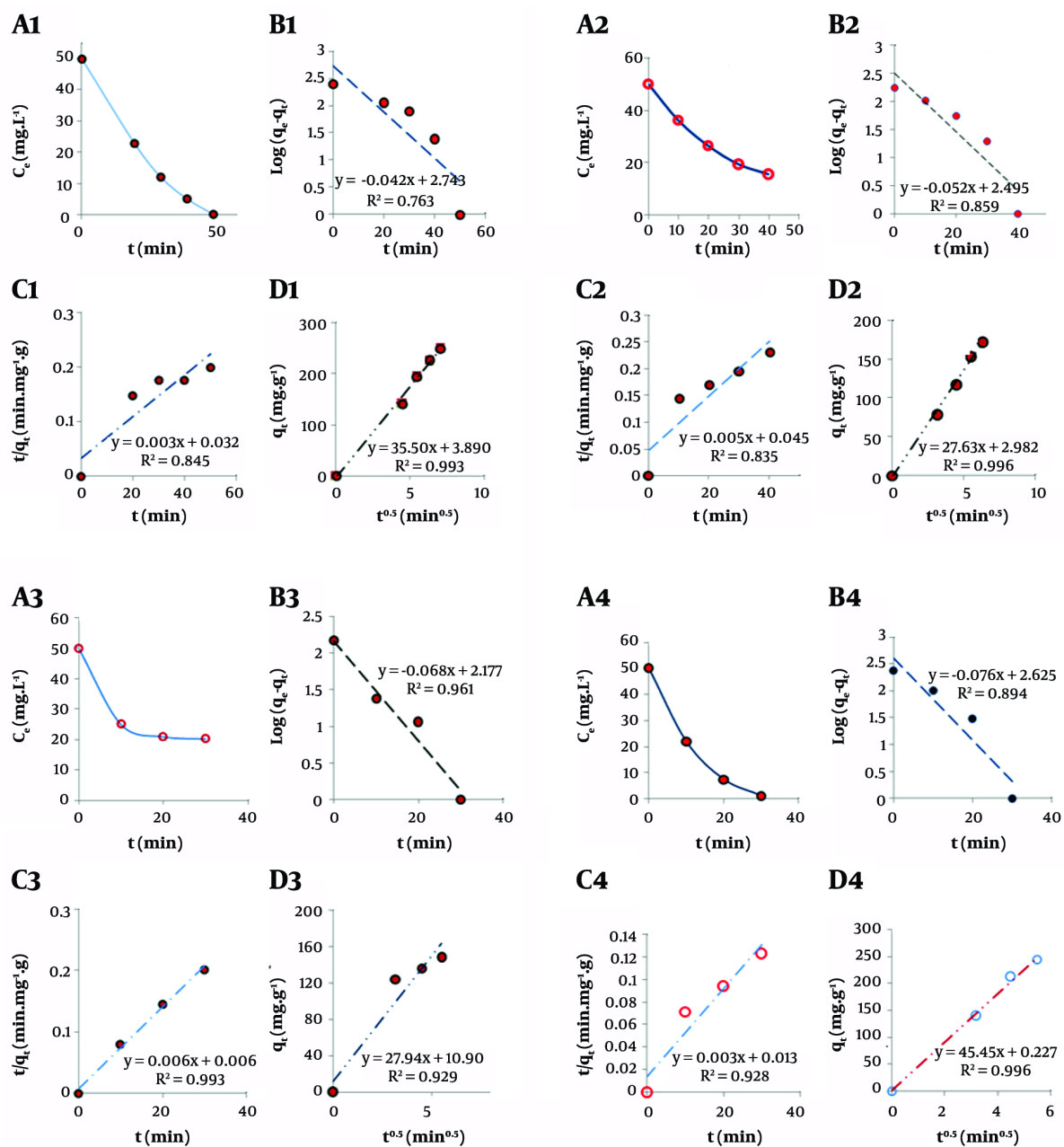
Figure 5. Kinetic models for the adsorption of chloroform on ZnO/GO, (a1-a4) concentration-time profile of chloroform removal, (b1-b4) pseudo-first-order model, (c1-c4) pseudo-second-order model, and (d1-d4) inter-particle diffusion model for ZnO/GO, ZnO, ZnO/GO/Zeolite, and GO/Zeolite, respectively
