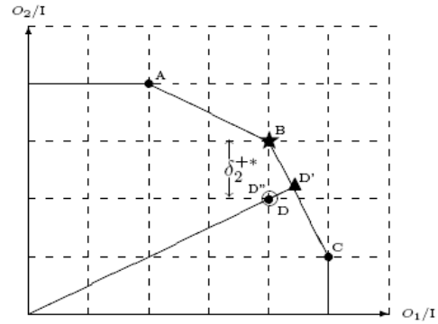
Fig. 2. Integer target setting constant input and two output case
