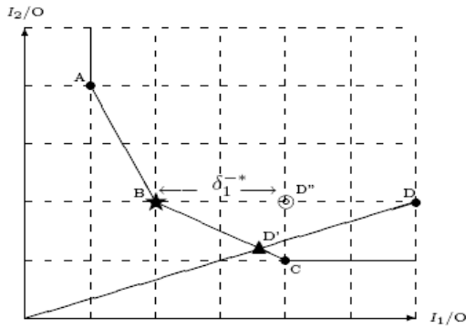
Fig. 1. Integer target setting constant output and two case
