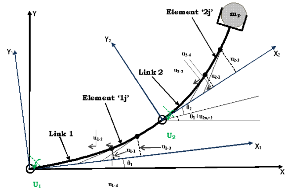
Fig. 1. A two-link manipulator with flexible links.
