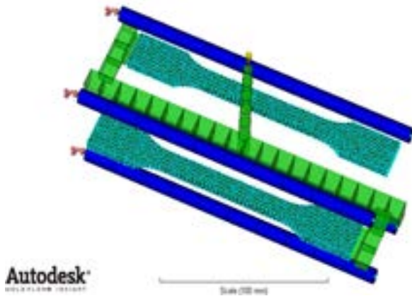
Fig.3. Part and runner system modeled and meshed in MoldFlow
