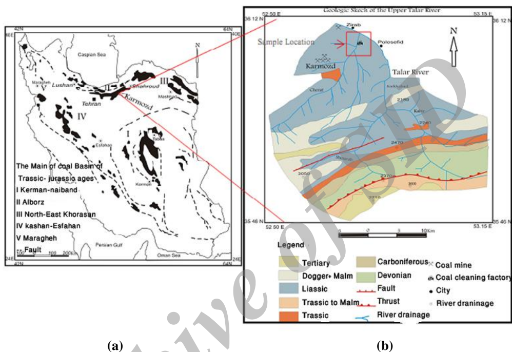
Figure 1. a: Situation of Zirab coal washing plant located in north of Iran; b: geological map of Talar watershed [15].
