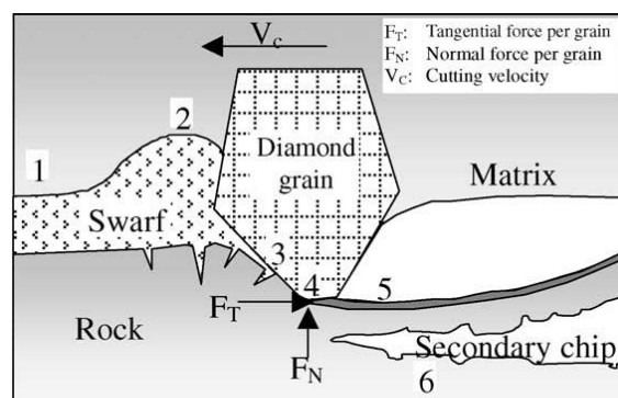
Figure 1. Mechanical interaction between saw and stone during sawing process [21].
