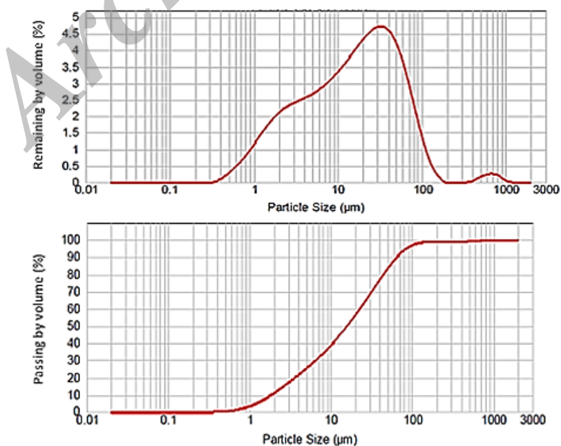
Figure 1. Size distribution of granite sludge.
