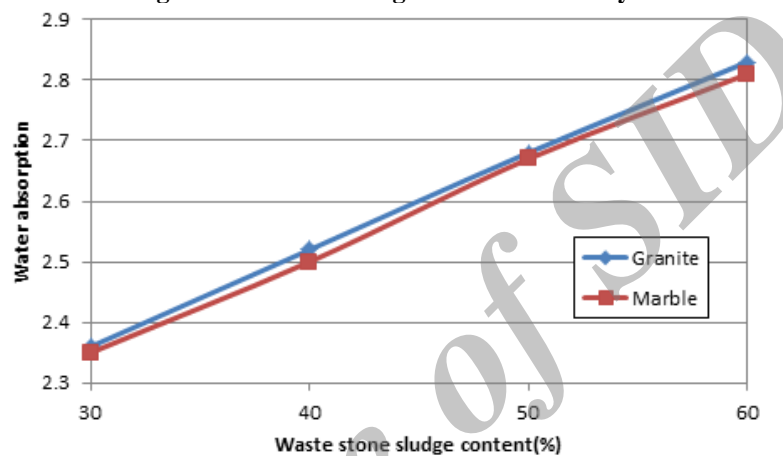
Figure 5. Effect of sludge content on water absorption.
