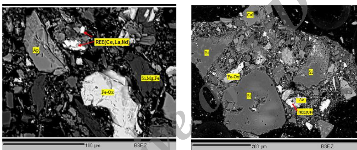
Figure 1. Back scattered electron (BSE) images by EPMA of iron waste.
