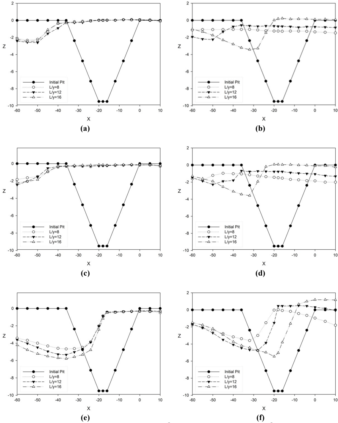
Figure 4. Sediment transport pattern a) upstream and \frac{S}{B} = 50\% , b) downstream and \frac{S}{B} = 50\% , c) upstream and \frac{S}{B} = 35\% , d) downstream and \frac{S}{B} = 35\% , e) upstream and \frac{S}{B} = 20\% , f) downstream and \frac{S}{B} = 20\% (flow direction is from right to left).
