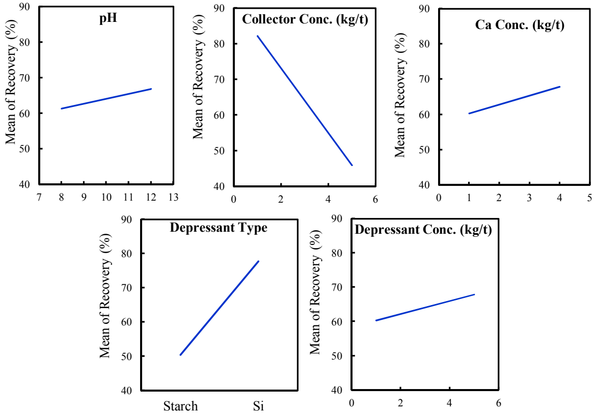
Figure 13. The effect of process parameters on the iron recovery in the reverse flotation process.
