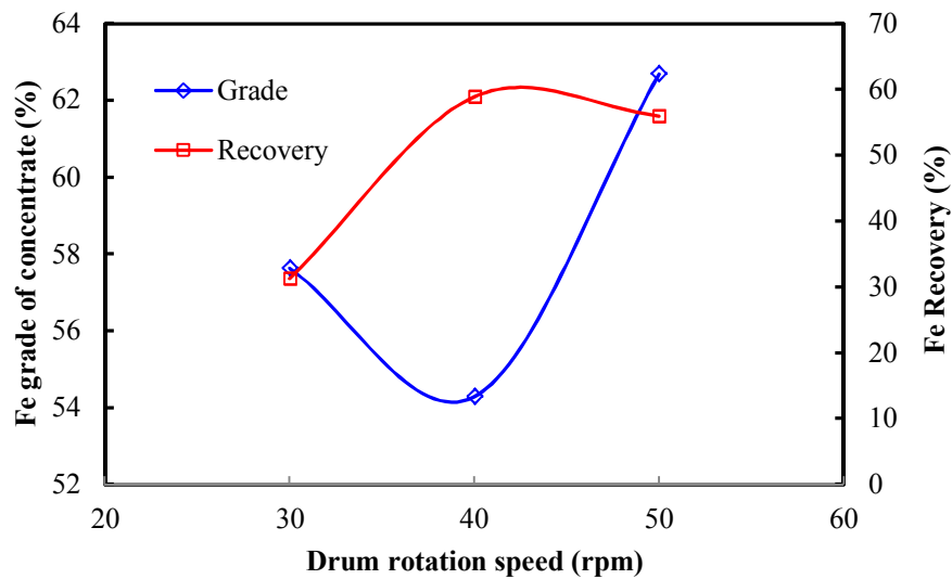
Figure 7. The effect of drum rotation speed on the performance of wet low-intensity magnetic separator.
