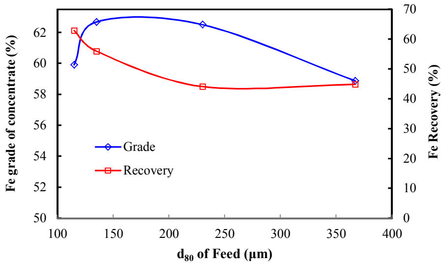
Figure 6. The effect of feed size on the performance of wet low-intensity magnetic separator.
