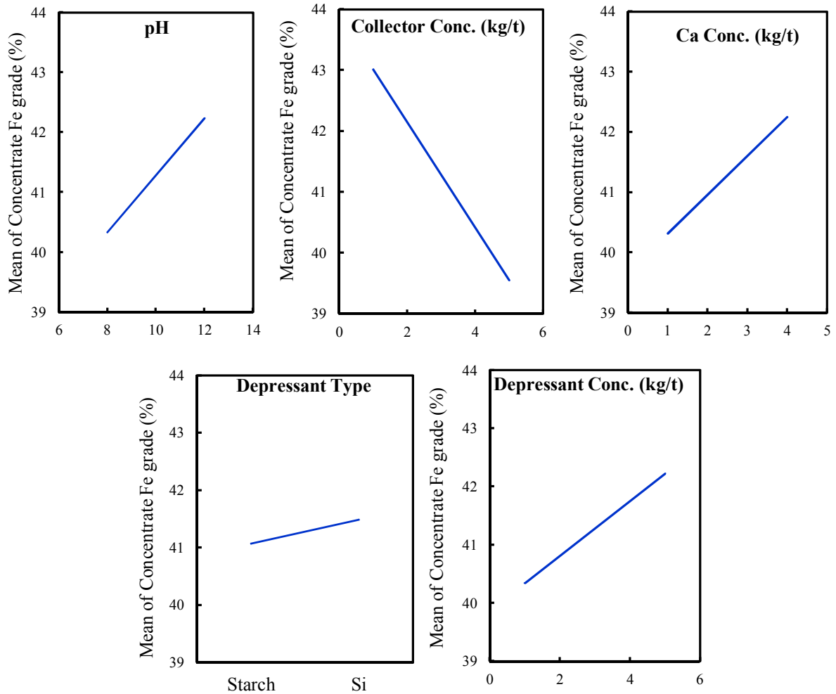
Figure 9. The effect of process parameters on the iron grade of reverse flotation concentrate.
