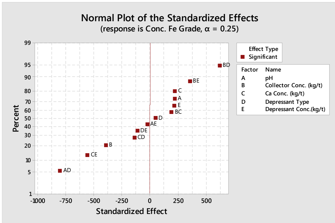
Figure 12. The normal plot for the main effects and their two-way interactions investigated on the iron grade of reverse flotation concentrate.
