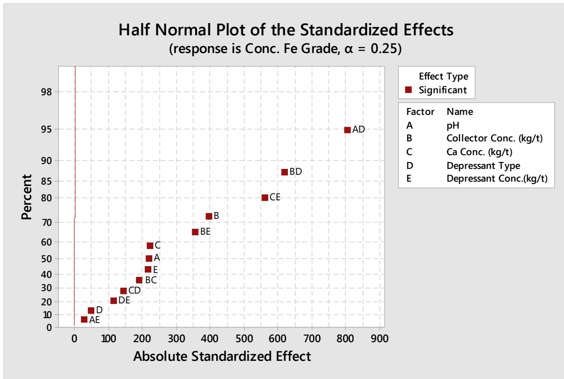
Figure 11. The half-normal plot for the main effects and their two-way interactions investigated on the iron grade of reverse flotation concentrate.
