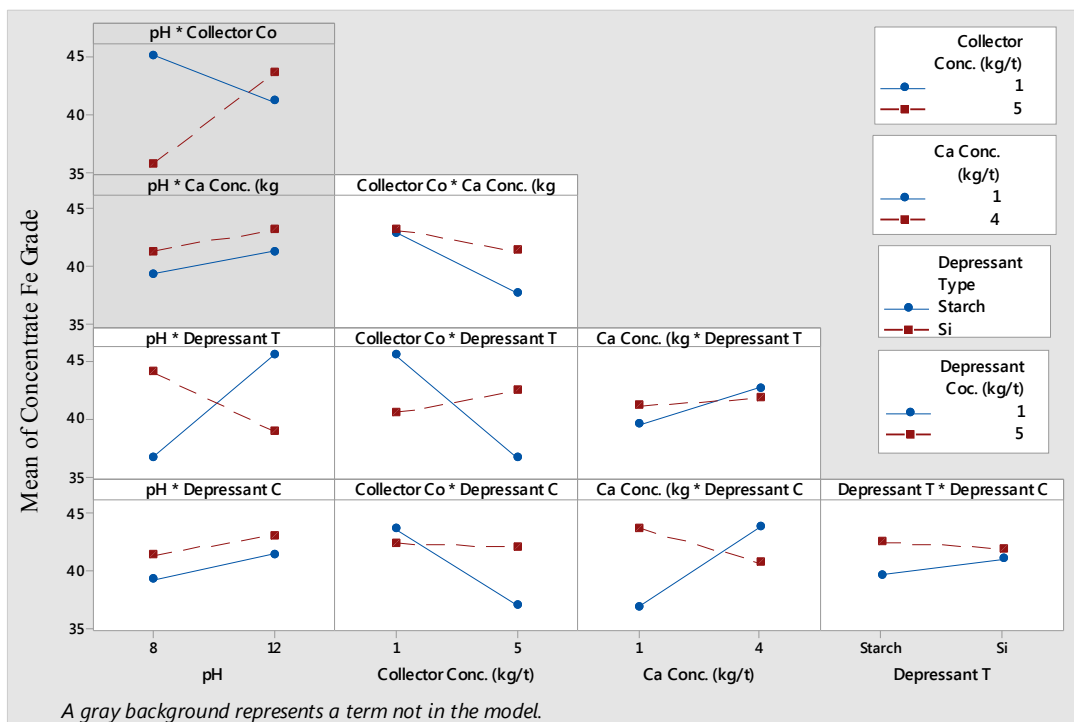
Figure 10. The two-way interactions between the factors investigated on the iron grade of reverse flotation concentrate.
