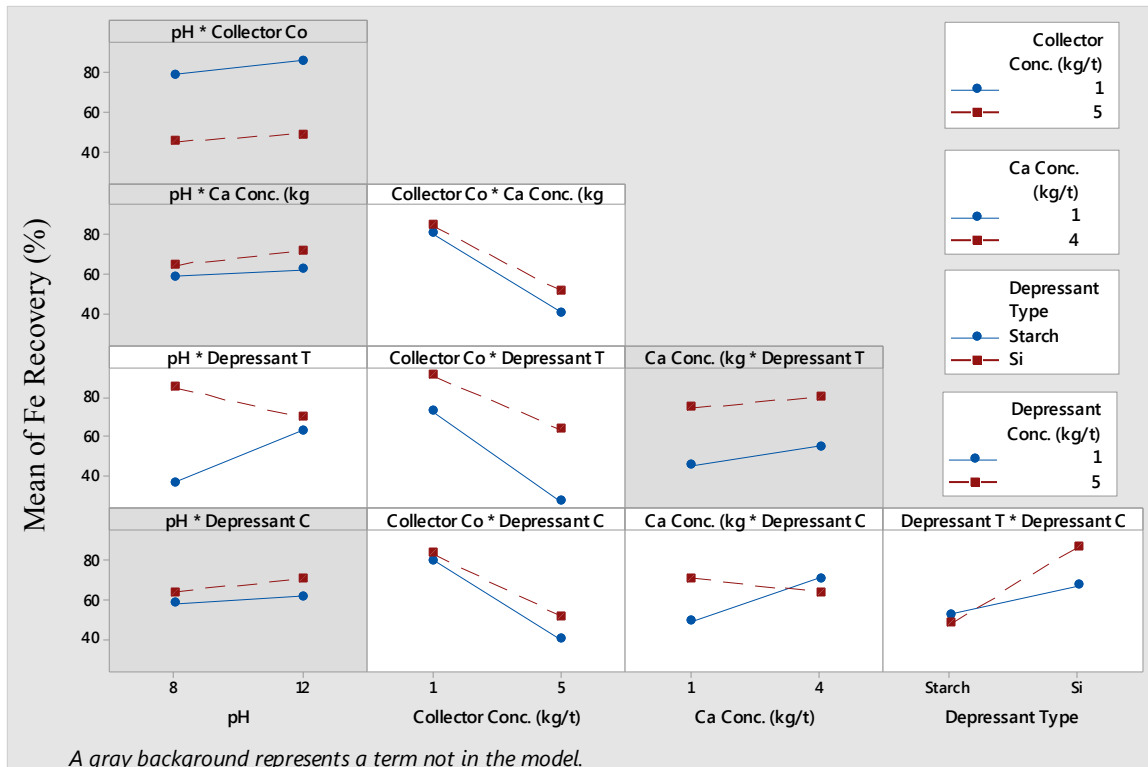
Figure 14. The two-way interactions between the factors investigated on the iron recovery in the reverse flotation process.
