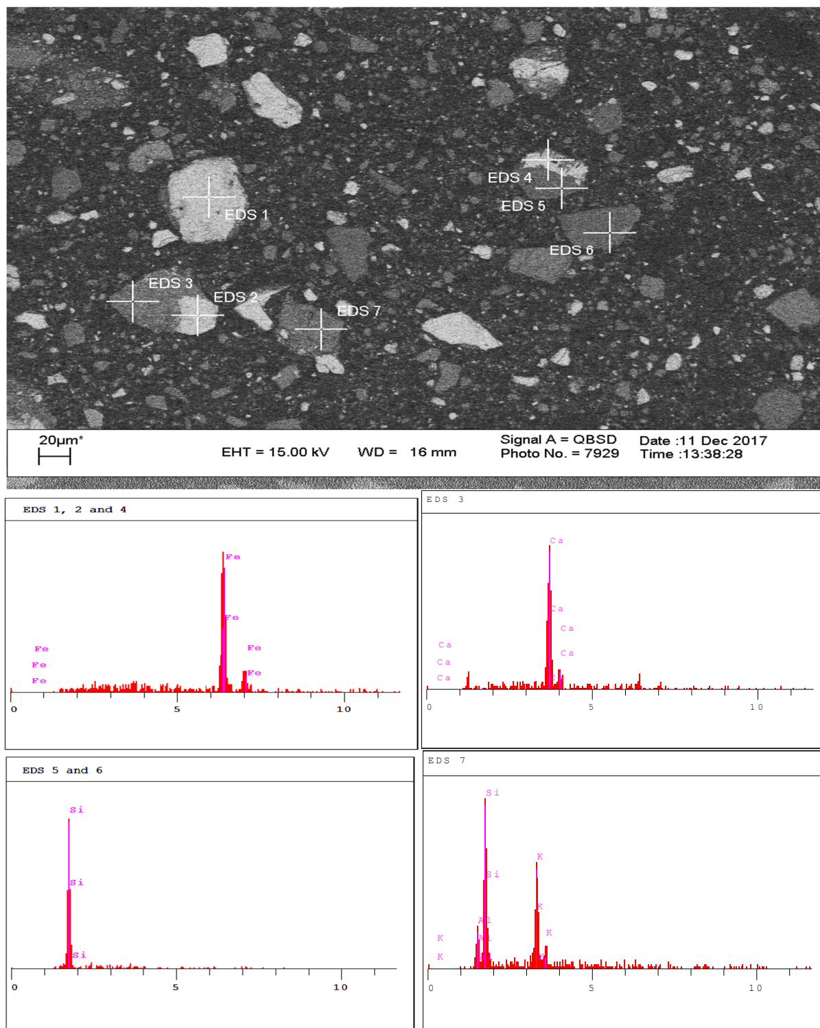
Figure 4. SEM-EDS analysis of the low-grade iron ore sample.
