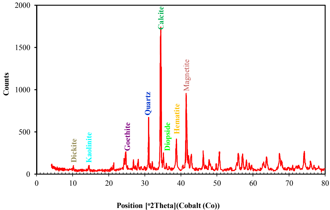
Figure 3. The XRD graph of the low-grade iron ore sample.
