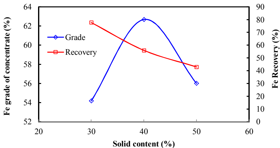
Figure 8. The effect of solid content on the performance of wet low-intensity magnetic separator.
