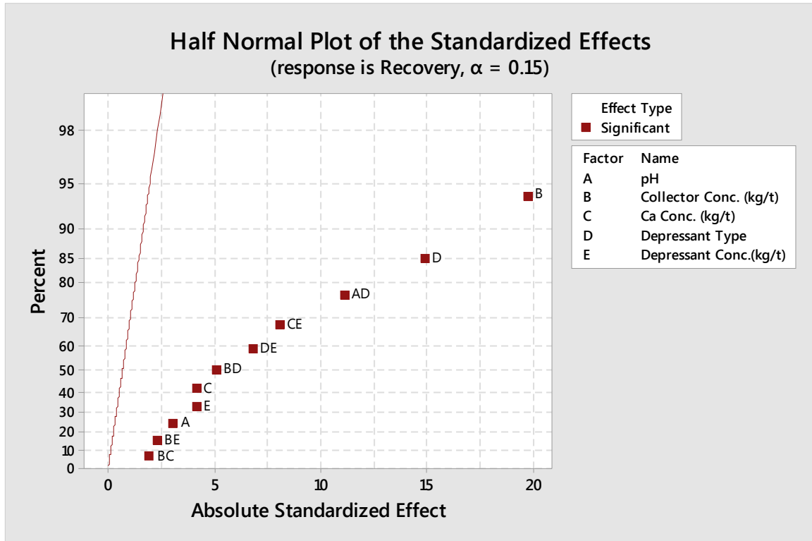
Figure 15. The half-normal plot for the main effects and their two-way interactions investigated on the iron recovery in the reverse flotation process.
