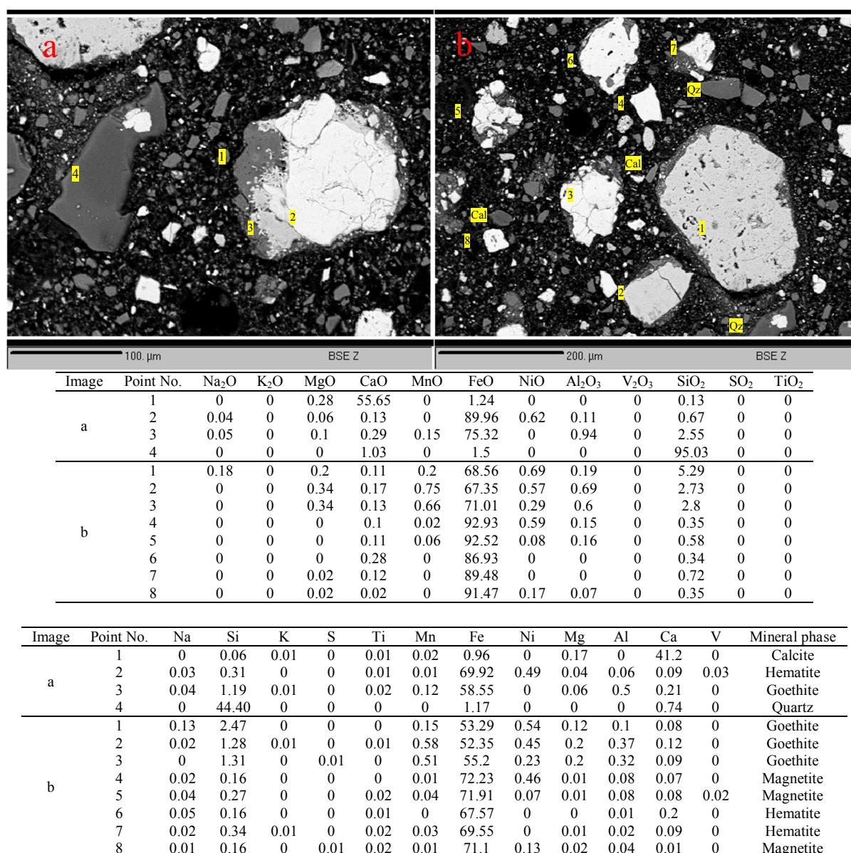
Figure 5. EPMA analysis of the sample.
