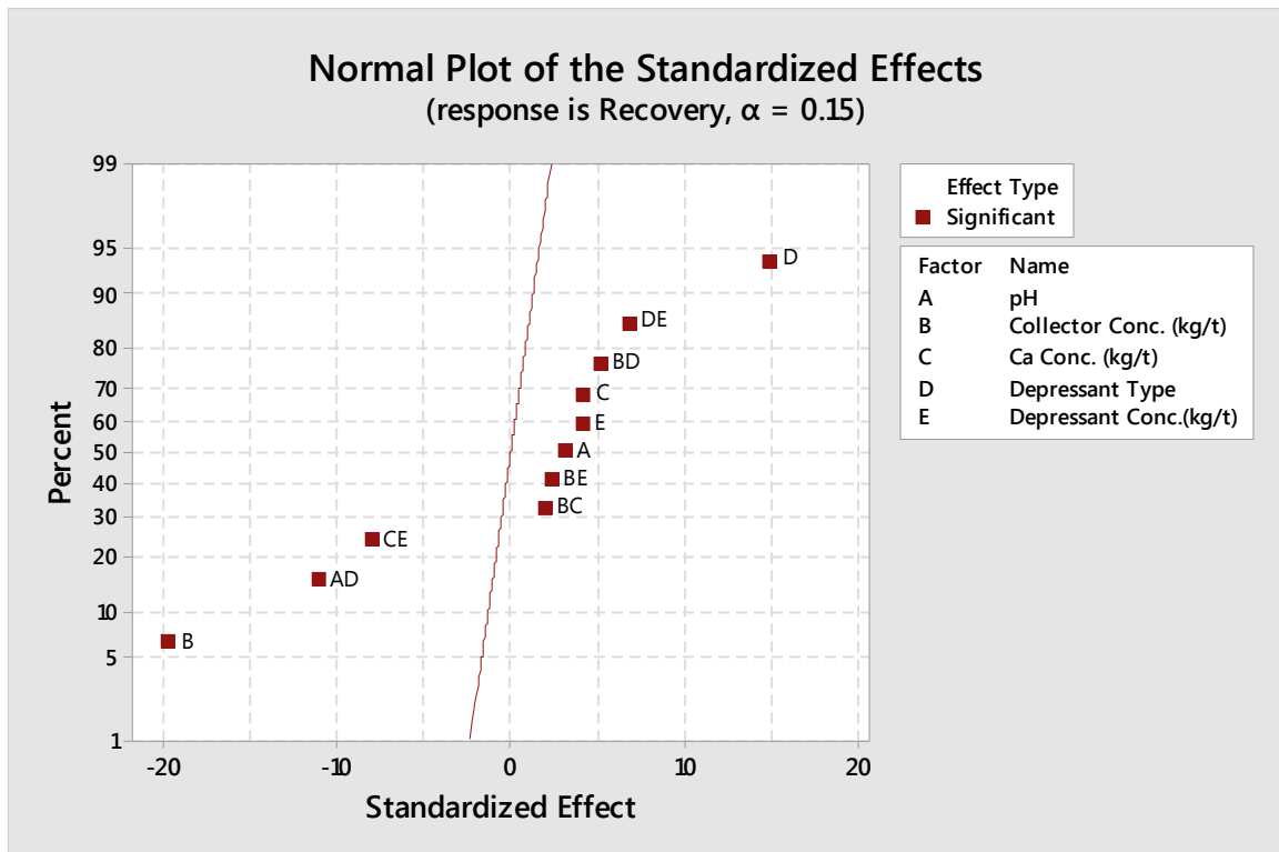
Figure 16. The normal plot for the main effects and their two-way interactions investigated on the iron recovery in the reverse flotation process.
