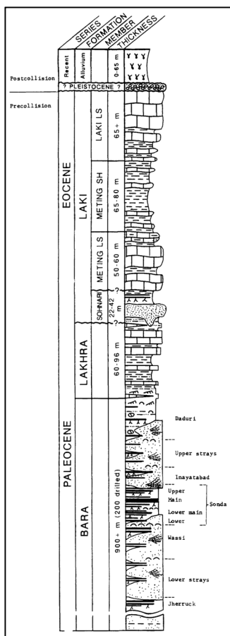
Figure 2. Stratigraphy column of the study area [20].
