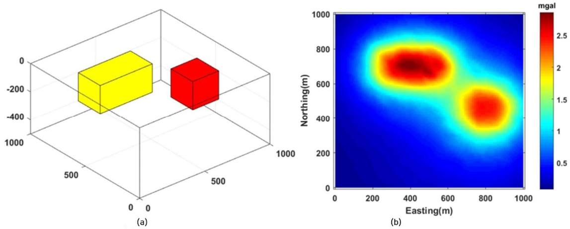
Figure 1. (a) Perspective view of the synthetic model. (b) Gravity anomaly produced by the synthetic model with 3% Gaussian noise.
