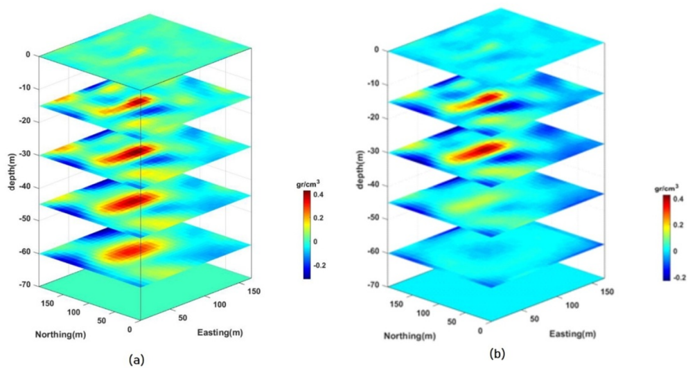
Figure 6. (a) Plan sections through the recovered density models obtained from the 3D smooth inversion of gravity anomaly using the GCV method at different depths. (b) The ACB method.
