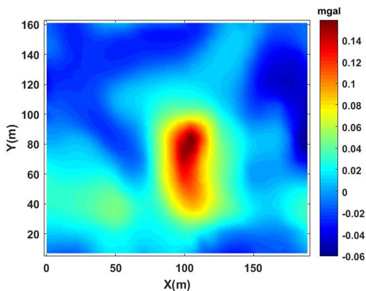
Figure 5. Holguin residual gravity map.
