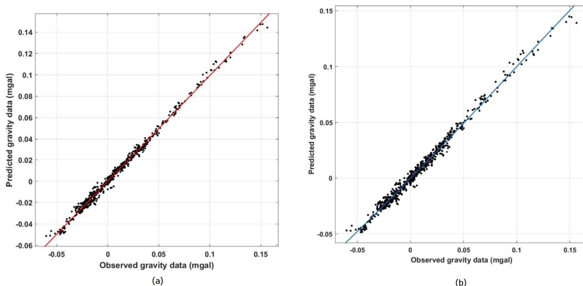
Figure 7. Data misfit between the predicted field gravity data with observed gravity data (a) GCV method. (b) ACB method.
