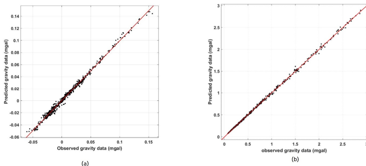
Figure 3. (a) Plot of the predicted gravity synthetic data versus the observed real data by the GCV method. (b) ACB method.
