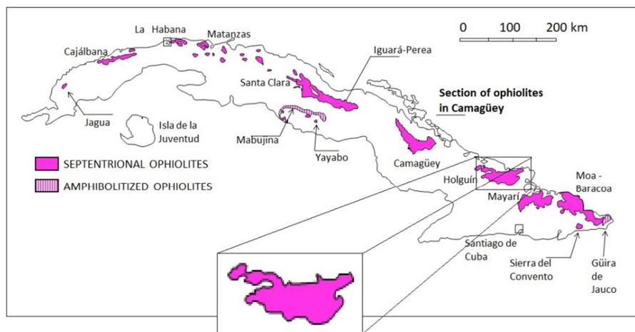
Figure 4. Distribution of ophiolites in the Holguin of Cuba.
