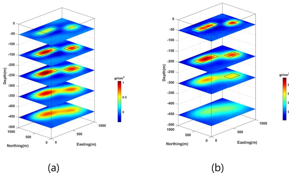
Figure 2. (a) Plan sections through the recovered density model obtained from inversion of gravity anomaly by the GCV method. (b) ACB method.
