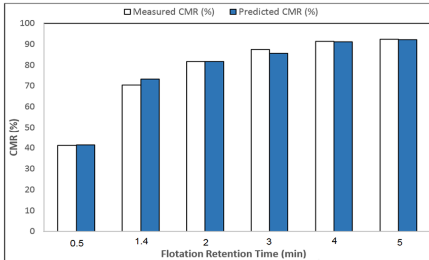
Figure 13. The predicted and experimental effects of flotation retention time on CMR: conditioning time, 3 min; gasoline dosage, 300 g/ton; pH, 8; MIBC dosage, 81 g/ton; solid weight content, 15%; rotor speed, 1200 RPM; and feed ash, 43.5%.
