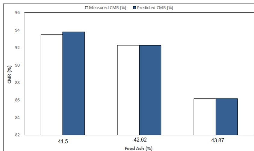
Figure 18. The predicted and experimental effects of feed ash on CMR: conditioning time, 3 min; rotor speed, 1200 RPM; pH, 8; flotation retention time, 3 min; collector dosage, 500 g/ton; frother dosage, 81g/ton; and solid weight content, 15%.
