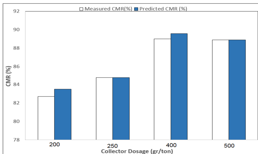
Figure 16. The predicted and experimental effects of gasoline (collector) dosage on CMR: conditioning time, 3min; rotor speed, 1200 RPM; pH, 8; flotation retention time, 3 min; solid weight content, 12%; frother dosage, 81 g/ton; and feed ash, 43.87%.
