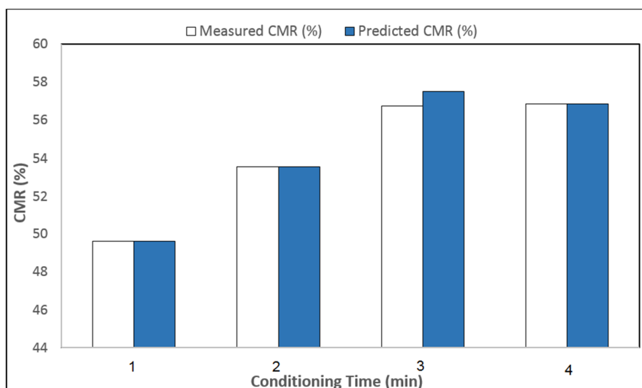
Figure 12. The predicted and experimental effects of conditioning time on CMR: pH, 8; gasoline dosage, 500 g/ton; flotation retention time, 4 min; MIBC dosage, 50 g/ton; solid weight content, 10%; rotor speed, 1200 RPM; and feed ash, 43.9%.
