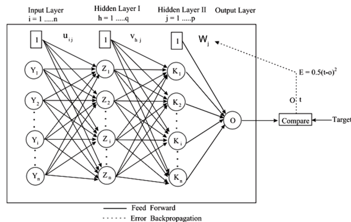
Figure 1. A flowchart of a typical two-hidden-layer BPNN [23].
