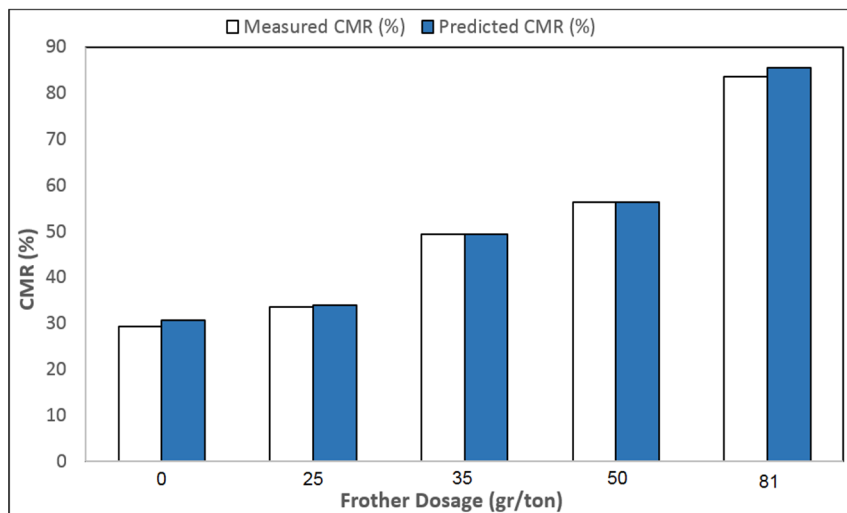
Figure 14. The predicted and experimental effects of MIBC (frother) dosage on CMR: conditioning time, 3 min; gasoline dosage, 300 g/ton; pH, 8; flotation retention time, 3 min; solid weight content, 15%; rotor speed, 1200 RPM; and feed ash, 43.6%.
