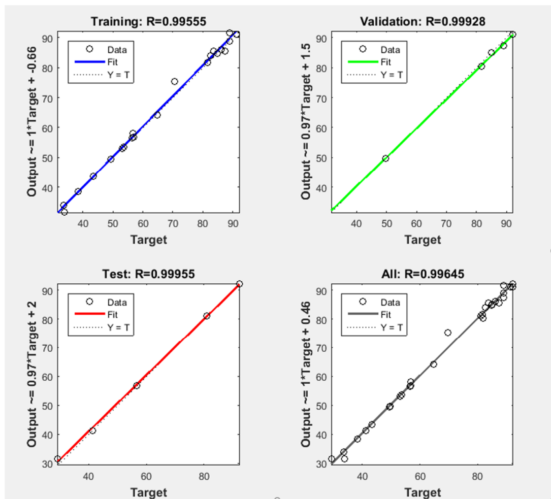
Figure 8. Correlation between the measured and predicted CM for training, testing, validation, and all data.
