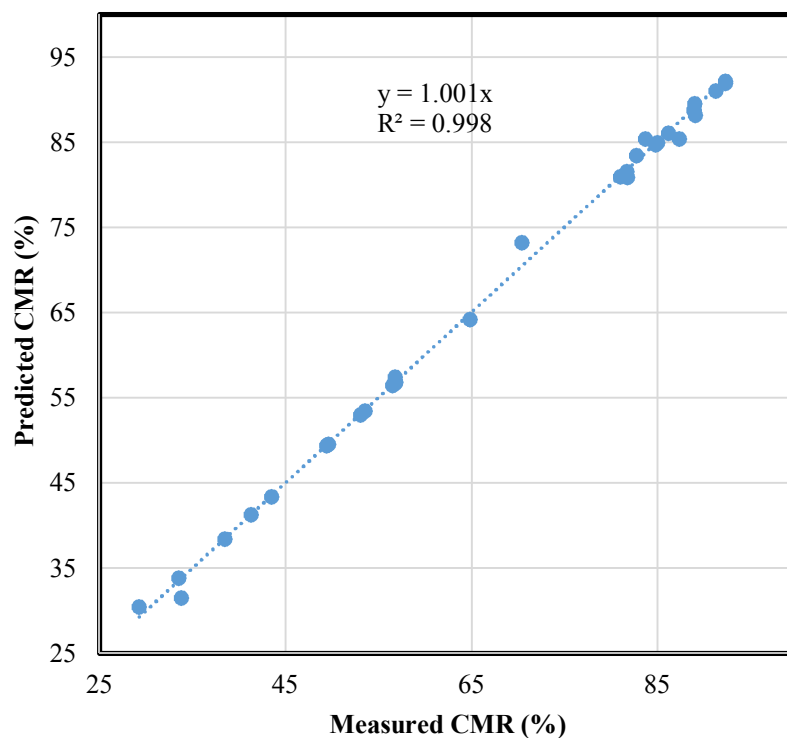
Figure 9. Correlation between the measured and predicted CMR for all data.
