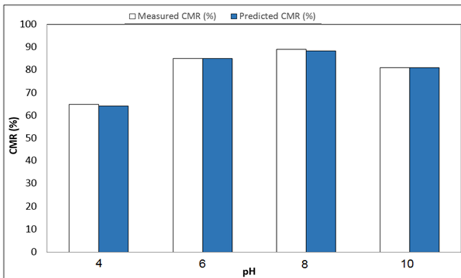
Figure 11. The predicted and experimental effects of pH on CMR: conditioning time, 3min; gasoline dosage, 500 g/ton; flotation retention time, 3 min; MIBC dosage, 50 g/ton; solid weight content, 12%; rotor speed, 1200 RPM; and feed ash, 43.5%.
