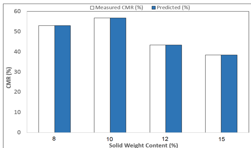
Figure 17. The predicted and experimental effects of solid weight content on CMR: conditioning time, 3 min; rotor speed, 1200 RPM; pH, 8; flotation retention time, 3 min; collector dosage, 250 g/ton; frother dosage, 50g/ton; and feed ash, 41.9%.
