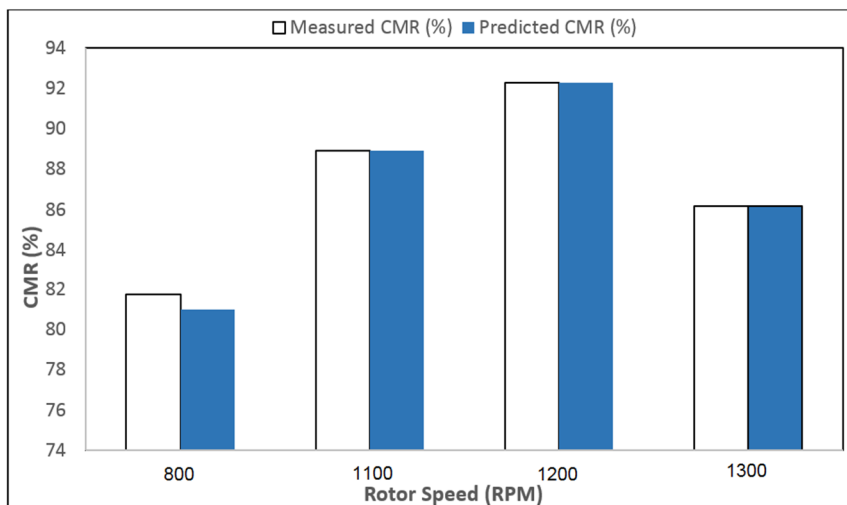
Figure 15. The predicted and experimental effects of rotor speed on CMR: conditioning time, 3 min; gasoline dosage, 300 g/ton; pH, 8; flotation retention time, 3 min; solid weight content, 15%; frother dosage, 25 g/ton; and feed ash, 43.9%.
