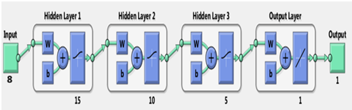
Figure 5. Architecture of the ANN model for coal flotation.
