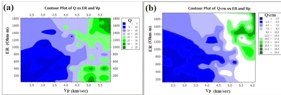
Figure 8. Contour plots of relation between V_p and ER with Q (a) and Q_{srm} (b).
