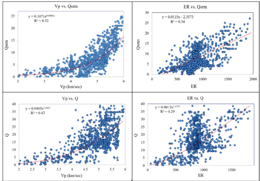
Figure 7. Regression analyses of relation between V_p , ER, Q and Q_{srm} .
