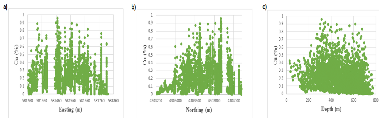
Figure 6. Variability of Cu concentration in a) east-west direction, b) north-south direction and c) depth within the hypogene zone of Masjed-Daghi deposit
