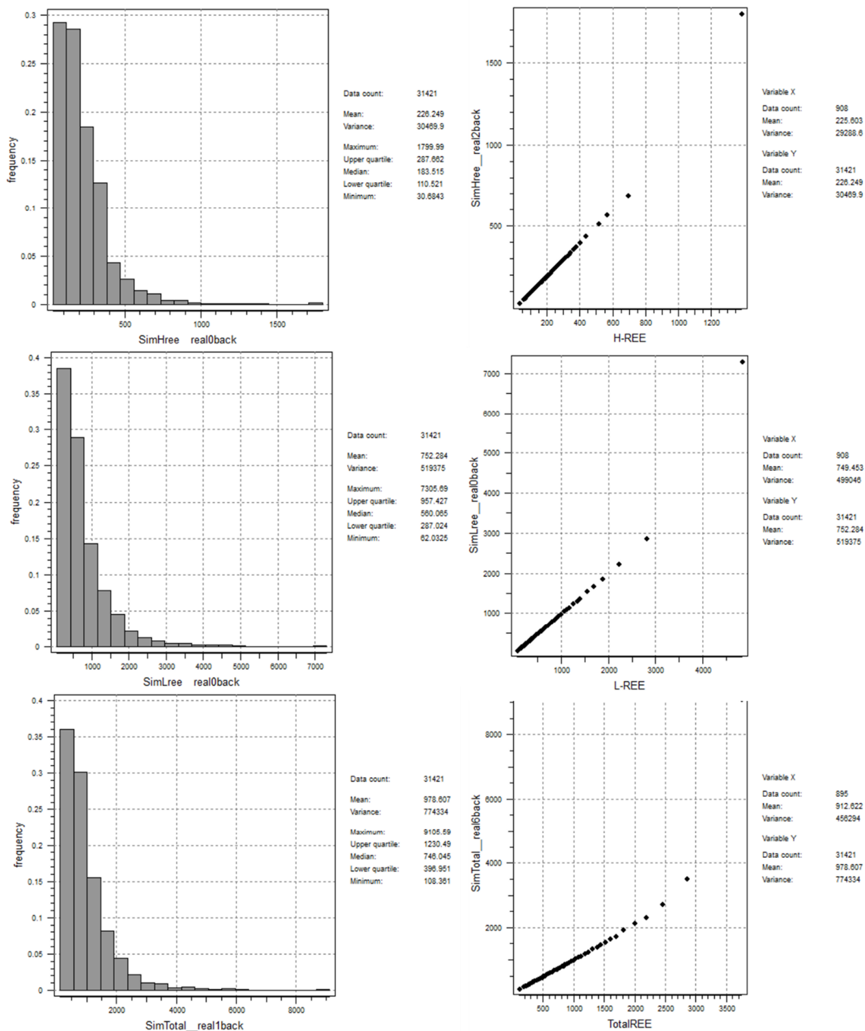
Figure 7. Histogram of the total, heavy, and light REEs of one realization along with the corresponding QQ diagram to be compared with the data distribution used in the simulation.
