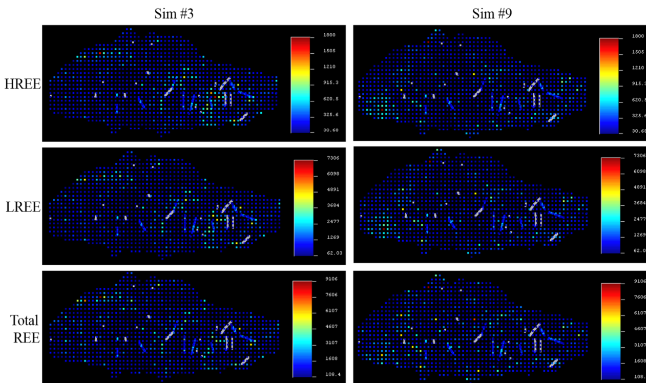
Figure 9. Plans of back-transformed variables into original distribution. Two random realizations (#3 and #9) have been shown for back-transformed HREE, LREE, and total REE.
