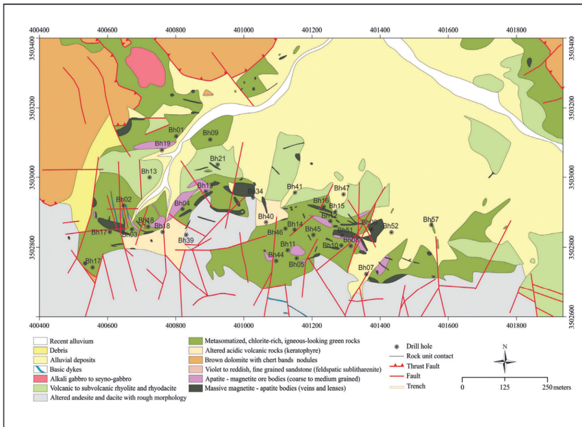
Figure 2. 1:1000 scale geology map of the Gezestan deposit [38].
