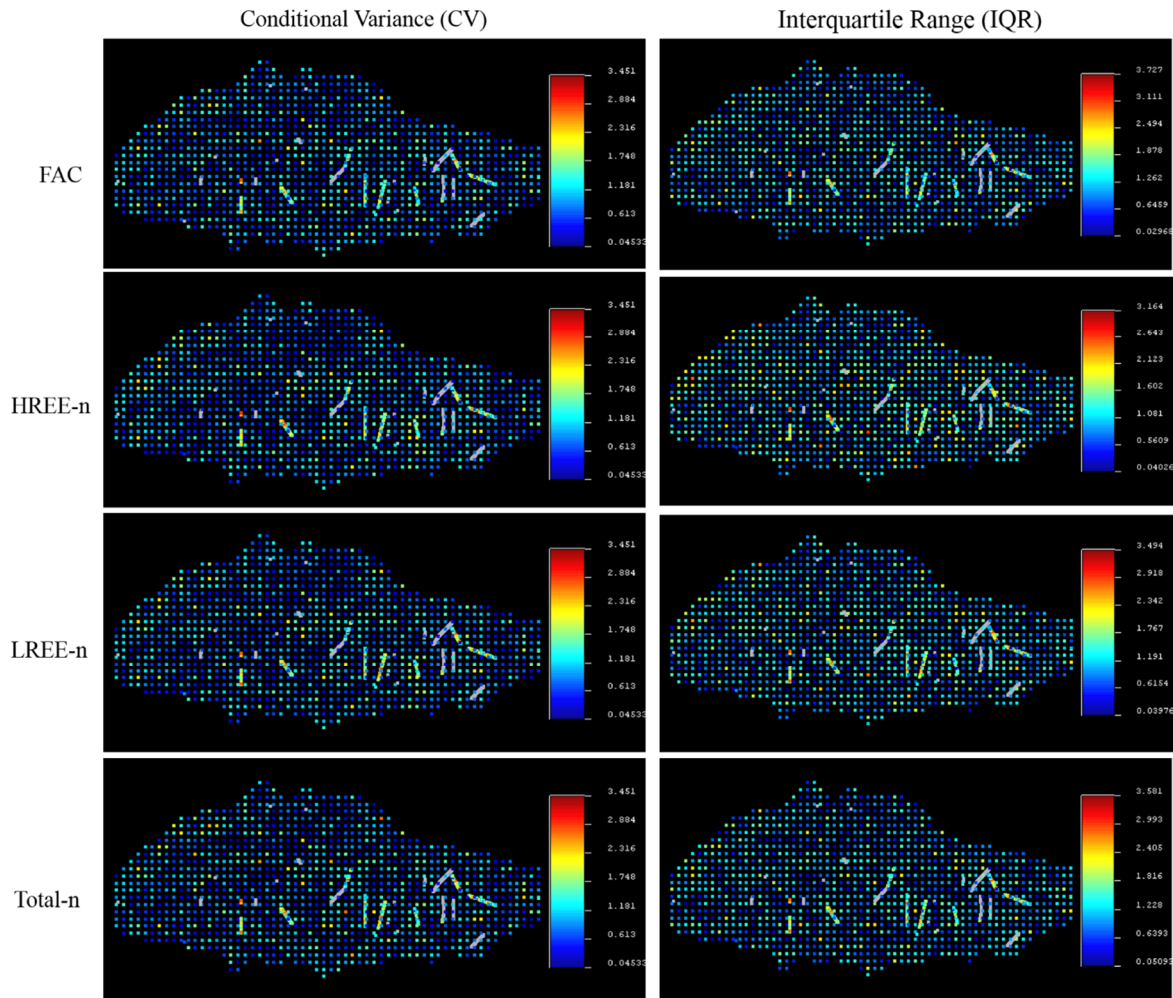
Figure 10. Quantification of uncertainty based on realizations of simulation for four variables including FAC, HREE, LREE and total REE. The right column is based on interquartile range (IQR) and the left one is based on conditional variance (CV).
