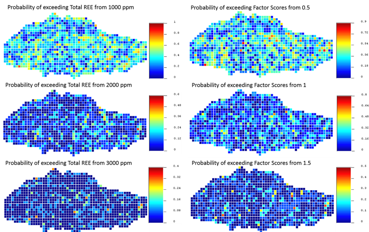
Figure 11. Maps of probability that the total REEs exceed 1000, 2000, and 3000 ppm, and that the corresponding factor scores exceed 0.5, 1, and 1.5.
