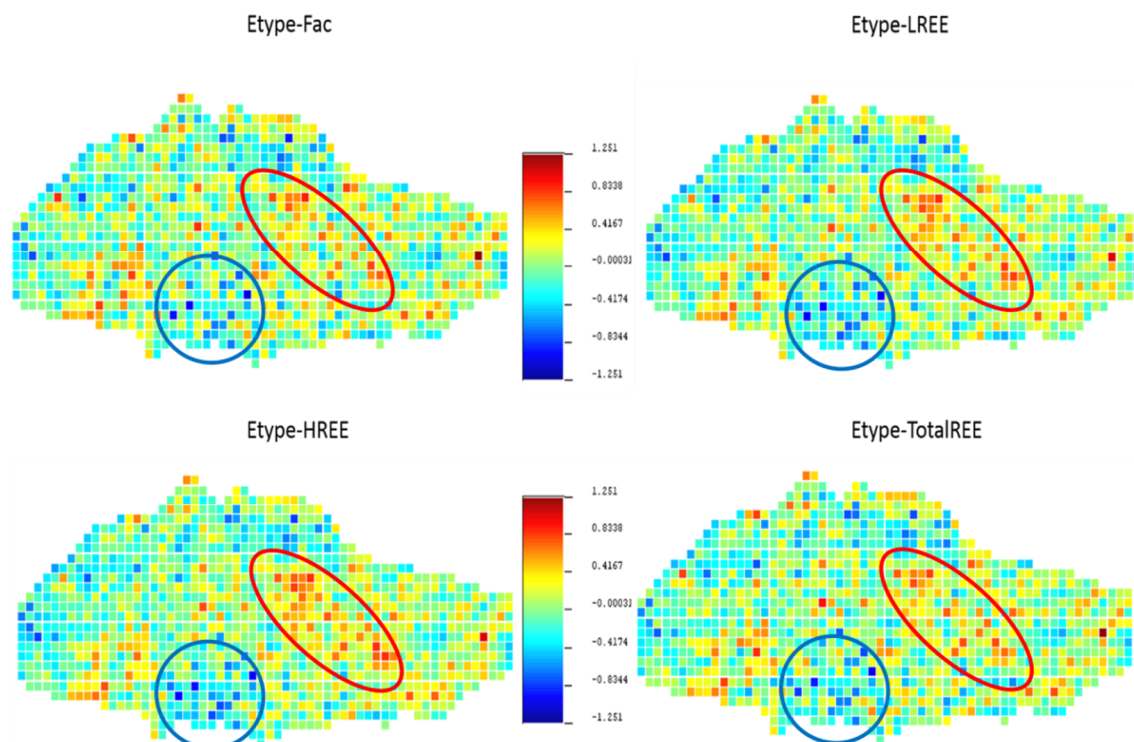
Figure 8. E-type map of factor values, heavy, light, and total REEs in Gaussian space.
