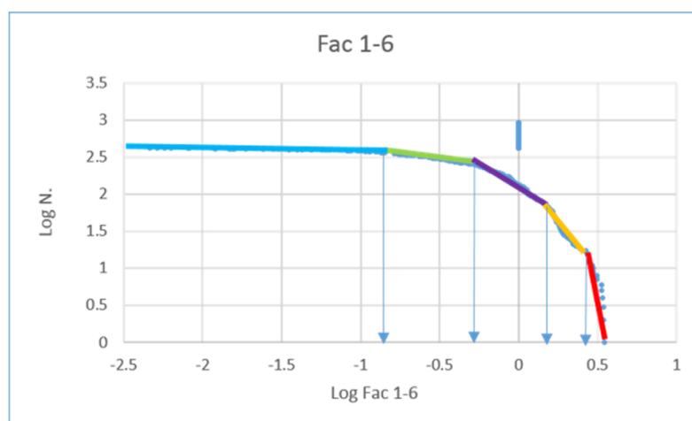
Figure 4. C-N logarithmic diagram of scores of the first factor from the 6 th stage of the staged factor analysis and the corresponding break points.
