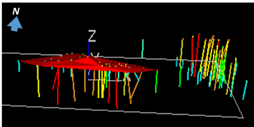
Figure 3. Western drilled boreholes of the Gazestan deposit utilized for further simulation. View to the North.
