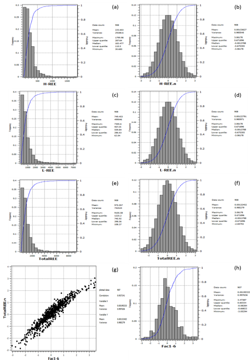
Figure 5. Histograms of a. HREE, c. LREE, and e. total REE on the left and the corresponding normalized values on the right. Scatter plot between the total normalized concentration values and the mineralization factor (g), histogram of the mineralization factor (h).
