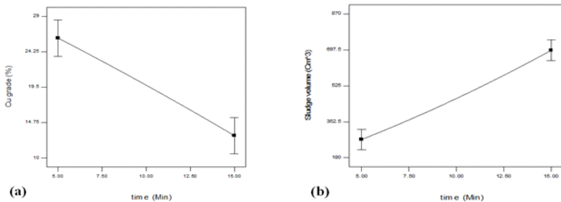
Figure 8. Effect of time a) on Cu grade (%) and b) on sludge volume (electrode type: Fe-Al; current density: 104.10; initial pH: 7), One factor plot
