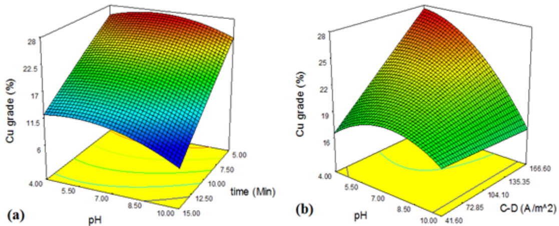
Figure 4. Effect of a) initial pH and electrolysis time, (electrode type: Fe-Al; current density: 104.10) and b) initial pH and current density (electrode type: Fe-Al; electrolysis time: 10 min) on Cu grade (%), 3D surface plots.
