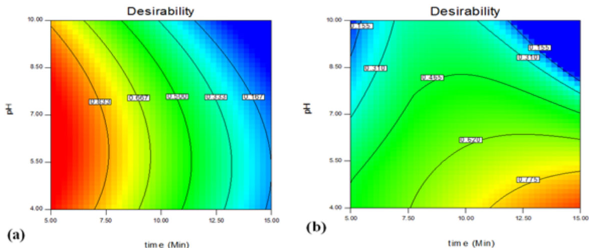
Figure 9. Desirability to obtain (a) Maximum Cu grade and (b) Maximum sludge volume (electrode type: Fe-Al; current density: 104.10), 2D contours.
