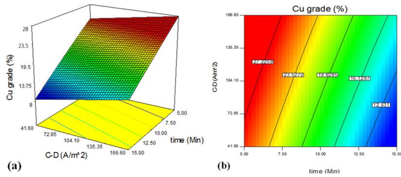
Figure 6. Effect of current density and electrolysis time on Cu grade (%), a) 3D plots and b) 2D contours.
