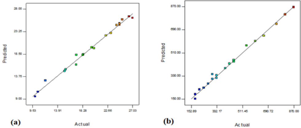
Figure 2. The actual and predicted plot for (a) Cu grade and (b) sludge volume.
