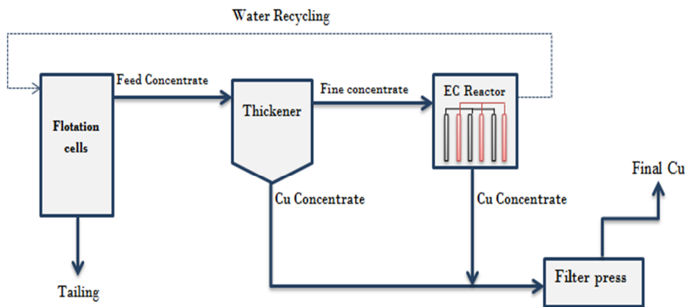
Figure 1. Experimental circuit.
