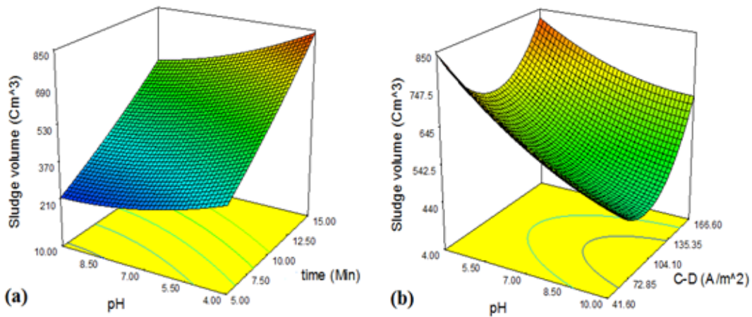
Figure 5. Effect of a) initial pH and electrolysis time (electrode type: Fe-Al; current density: 104.10), and b) initial pH and current density (electrode type: Fe-Al; electrolysis time: 10 min) on sludge volume (Cm³); 3D surface plots.
