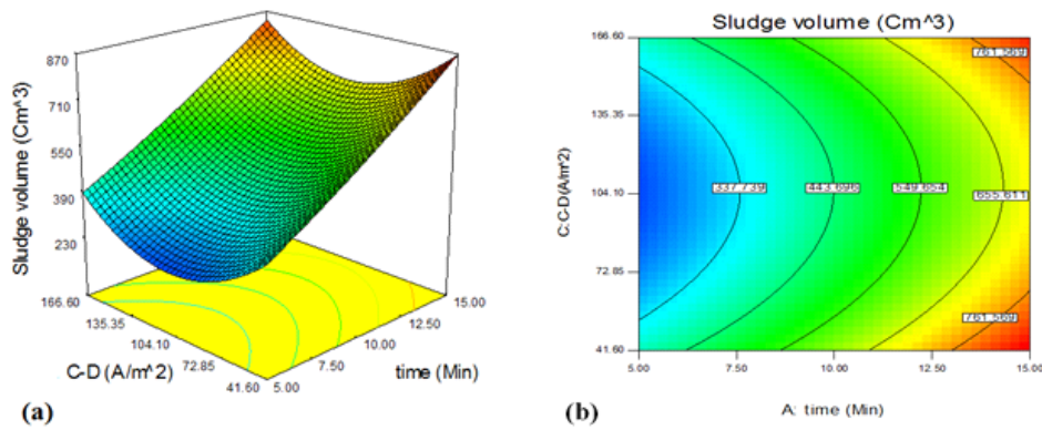
Figure 7. Effect of current density and electrolysis time on sludge volume, a) 3D plots and b) 2D contours.
