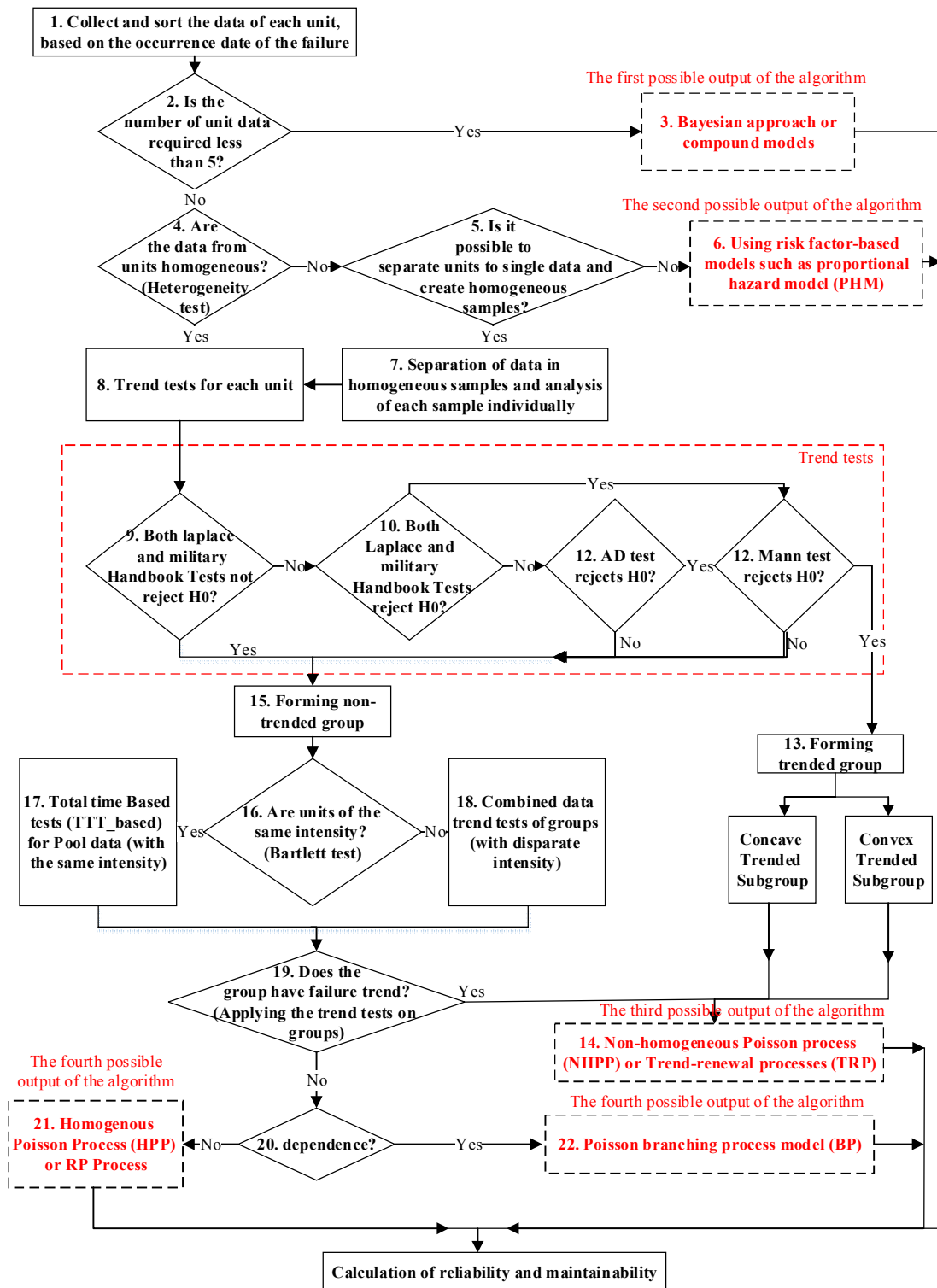
Figure 1. Main framework of reliability and maintainability of multi-component units.
