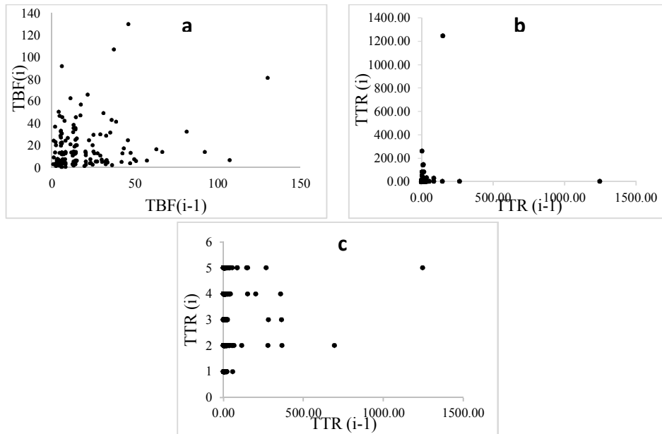
Figure 2. a) Serial-correlation test of group loader 1 (TBF), b) serial-correlation test of group loader 1 (TTR), c) serial-correlation test of group dump trucks 2, 3, 4, 5, 8 (TTR).
