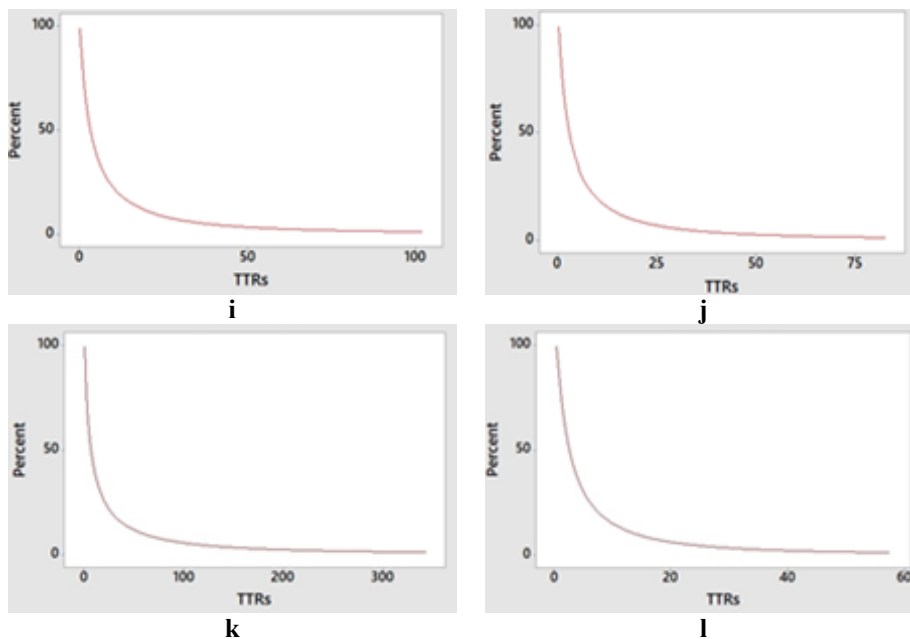
Figure 4. i) Maintainability function of group loader 1, j) maintainability function of group dump trucks 1, 6, 7, k) maintainability plot for group loader 1, l) maintainability plot for group dump trucks 2, 3, 4, 5, and 8, respectively.
