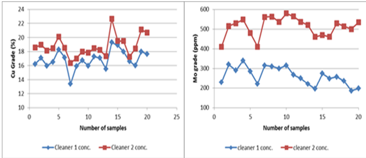
Figure 7. Concentrate grade comparison in column cells of No. 1 and No. 2.
