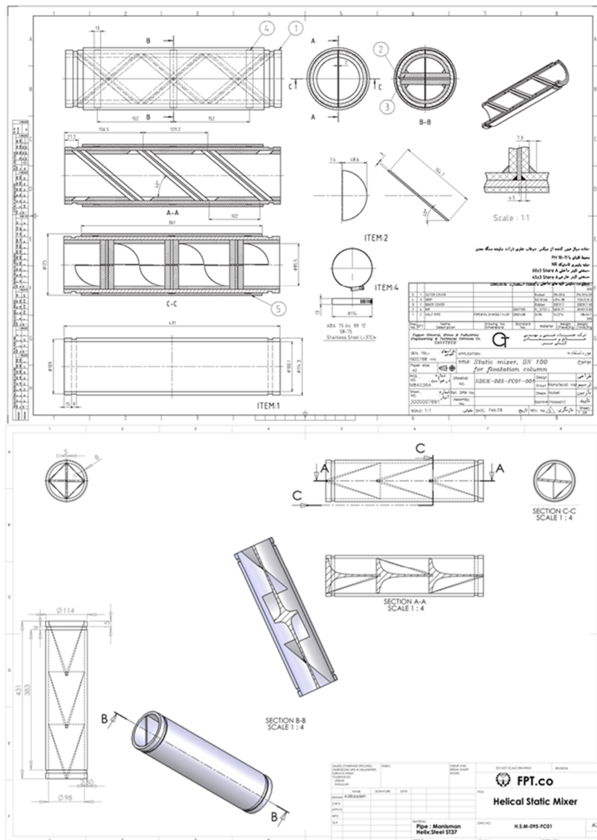
Figure 1. Technical design of elliptical (left) and helical (right) static mixers.
