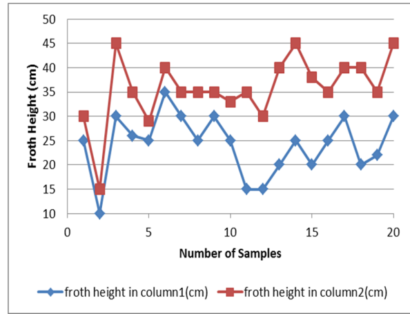
Figure 4. Froth depth in helical column cell vs. elliptical column cell during 60 days continuous monitoring.
