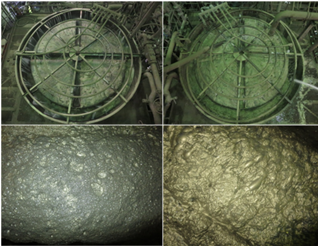
Figure 2. The froth generated in elliptical column cells (right) and helical column cells (left).
