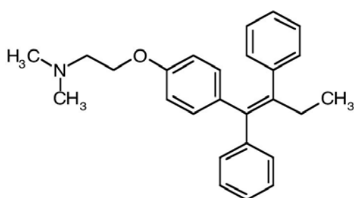
Fig. 1. The schematic diagram of Tamoxifen structure that interacted to SWNT.
