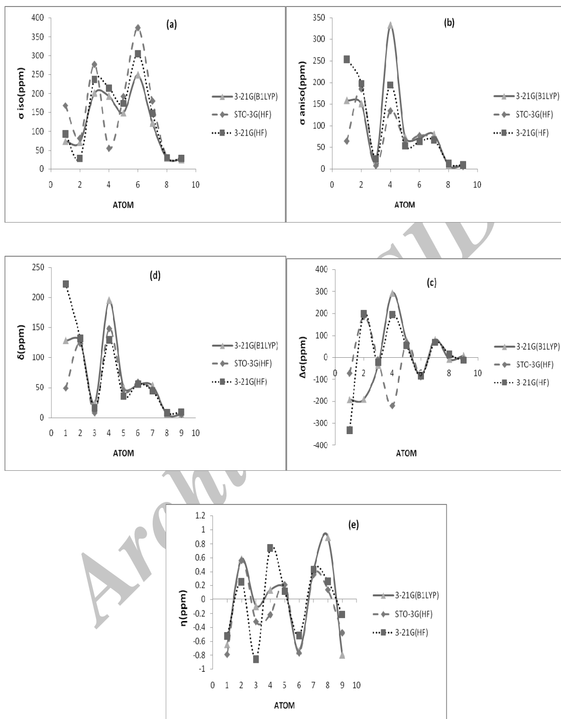
Fig. 3. The graphs of a) isotropic shielding values ( \sigma_{iso} ), b) anisotropic shielding value ( \sigma_{aniso} ), c) indirect shielding ( \Delta\sigma ), d) chemical shift tensor ( \delta ), e) asymmetry parameters ( \eta ), of propose atoms of active site tamoxifen interaction with open-end of SWNT, in water at the levels of HF/STO-3G, HF/3-21G and B1LYP/3-21G theories in GIAO method.
