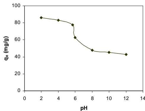
Fig. 3. Effect of pH on 4C2NP adsorption onto nano-TiO 2 (nano-TiO 2 dose: 0.01 g, initial 4C2NP conc.: 10 mg/L, temp.: 25°C, contact time: 1 h).
