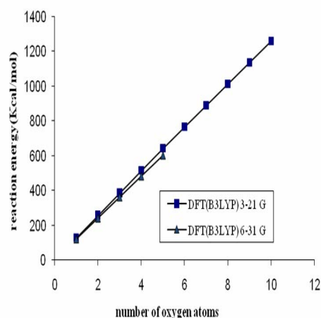
Fig. 11. The effect of 3-21G and 6-31G basis sets with DFT (B3LYP) method on reaction energy of carbon nanotube (10-0) with oxygen atoms.
