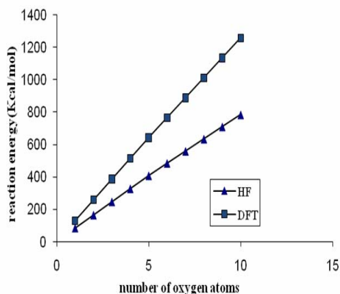
Fig. 8. The effect of HF/3-21G and B3LYP/3-21G on reaction energy of carbon nanotube(10-0) with oxygen atoms.
