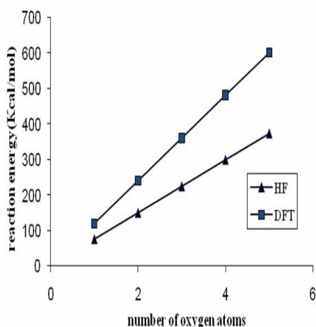
Fig. 9. The effect of HF/6-31G and B3LYP/6-31G on reaction energy of carbon nanotube (10-0) with oxygen atoms.
