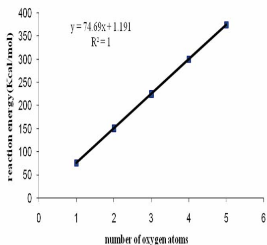
Fig. 6. Reaction energy curve for the adsorption of oxygen atoms with HF/6-31G.
