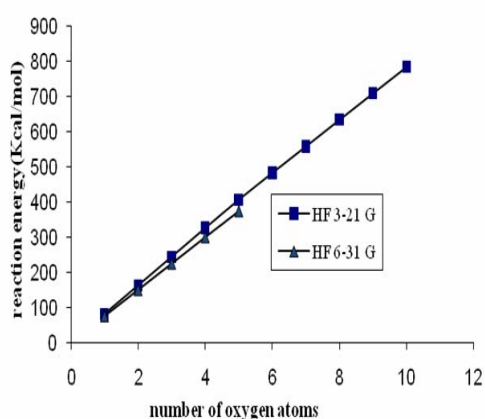
Fig. 10. The effect of 3-21G and 6-31G basis sets in HF method on reaction energy of carbon nanotube (10-0) with oxygen atoms.
