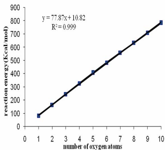
Fig. 4. Reaction energy curve for the adsorption of oxygen atoms with HF/3-21G.
