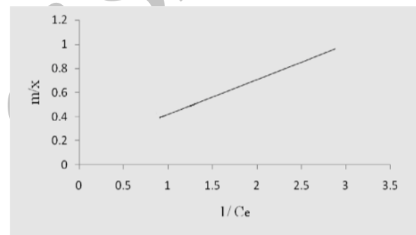
Fig. 8. Langmuir adsorption isotherm for the sorption of MG by PAni/SD.
