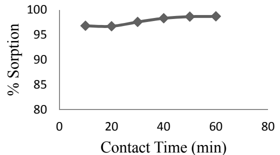
Fig. 7. Effect of contact time on the removal of MG by PAni/SD.
