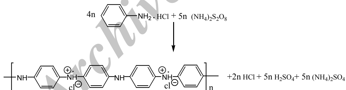
Fig. 2. Chemical polymerization of polyaniline.
