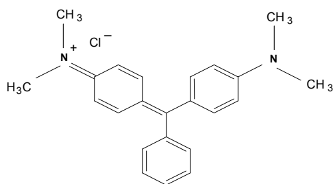
Fig. 1. Chemical structure of malachite green.
