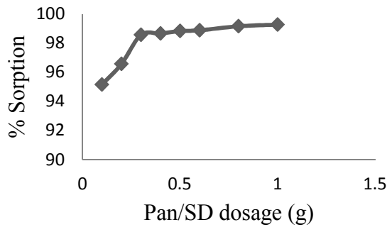
Fig. 6. Effect of amount of adsorbent on removal percentage of MG by PAni/SD.
