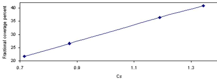
Fig. 5. The fractional coverage surface SHCL versus concentration of protein on the surface at pH 7.2 and 22°C.
