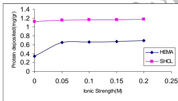
Fig. 2. The effect ionic strength of solutions on SHCL and HEMA surfaces, at pH 7.2 and 22°C concentration of protein is 1.2 mg/ml.
