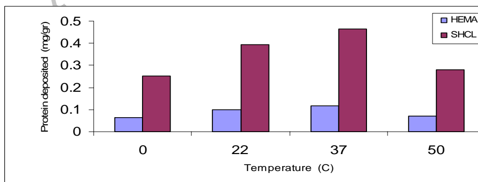
Fig. 6. The effect of temperature (°C) on protein adsorption on SHCL and HEMA surfaces, concentration of protein is 0.8 mg/ml at pH 7.2.
