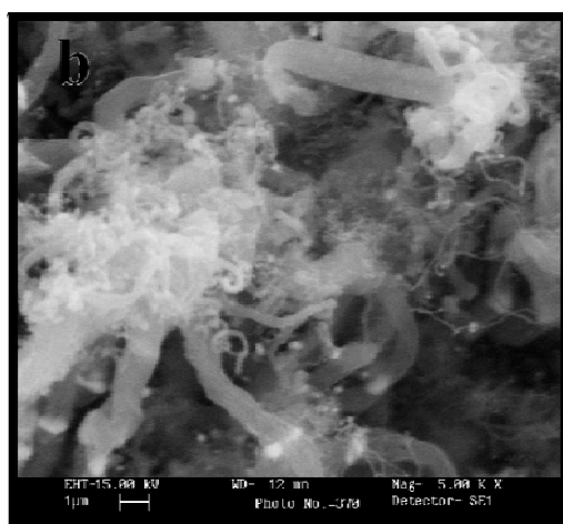
Fig. 2. SEM micrographs of carbon nanotubes deposited on stainless steel Substrates by (a) Co and (b) Ni catalysts.
