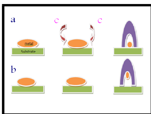
Fig. 3. Visualization of possible carbon nanotubes growth mechanisms of (a) root growth and (b) top growth.
