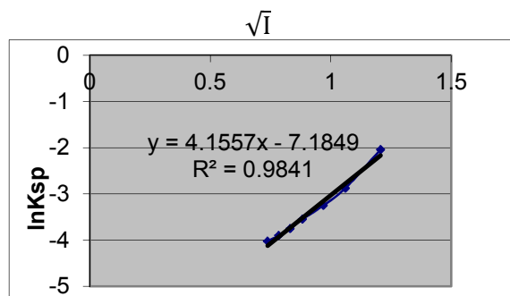
Fig.1. Plot of \ln K_{sp(c)} versus I^{1/2} in the mixed solvent (water 85%+ethanol 5% +propanol 10%) at 25^\circ C .
