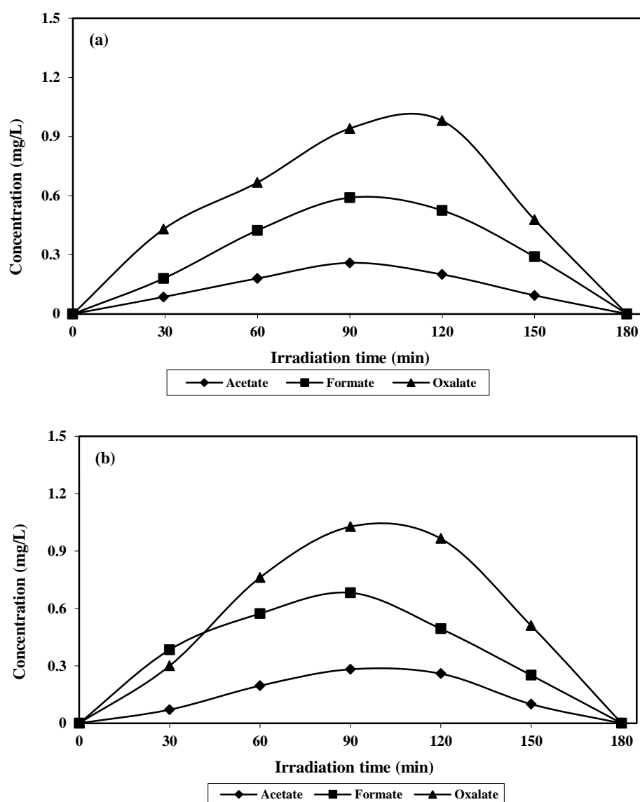
Figure 4: Formation and disappearance of aliphatic carboxylic acids during the photocatalytic ozonation of dyes (a) RRRB and (b) DGB (5 mg/L of NFN , Ozone concentration: 55 \text{ g/m}^3 , 1 L of dye solution (150 mg/L) and \text{pH}=3 at room temperature ( 25 \text{ }^\circ\text{C} )).
