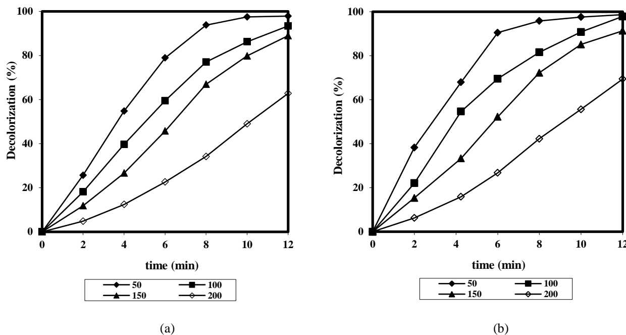
Figure 8: The effect of dye concentration (mg/L) on the decolorization of dyes using photocatalytic ozonation (a) RRRB and (b) DGB (5 mg/L of NFN, Ozone concentration: 55 \text{ g/m}^3 , and 1 L of dye solution at pH=3).
