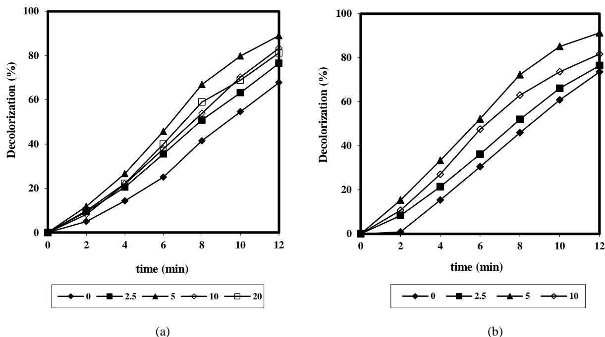
Figure 5: The effect of NFN dosage (mg/L) on the decolorization of dyes using photocatalytic ozonation (a) RRRB and (b) DGB (pH=3, Ozone concentration: 55 g/m 3 , and 1 L of dye solution (150 mg/L) at room temperature (25 °C)).
