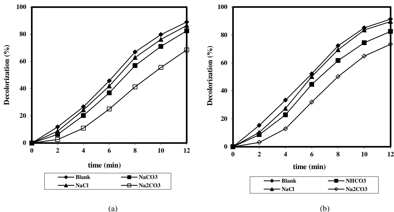
Figure 7: The effect of inorganic anions on the decolorization of dyes using photocatalytic ozonation (a) RRRB and (b) DGB (0.02 M of salts, Ozone concentration: 55 \text{ g/m}^3 , 5 mg/L of NFN and 1 L of dye solution (150 mg/L) at room temperature ( 25^\circ\text{C} )).
