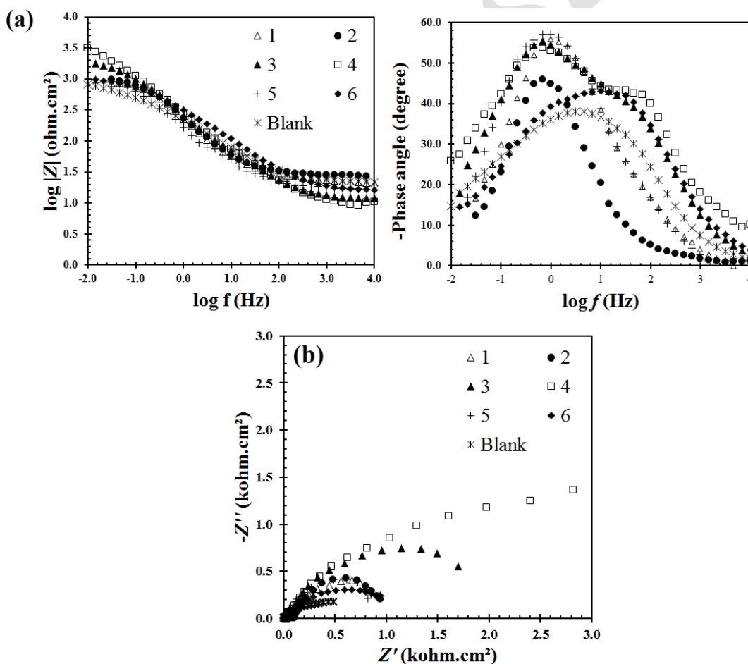
Figure 5: Typical Bode (a) and Nyquist (b) plots of the mild steel samples dipped in different test solutions (samples are defined in Table 3) for 4 h.
